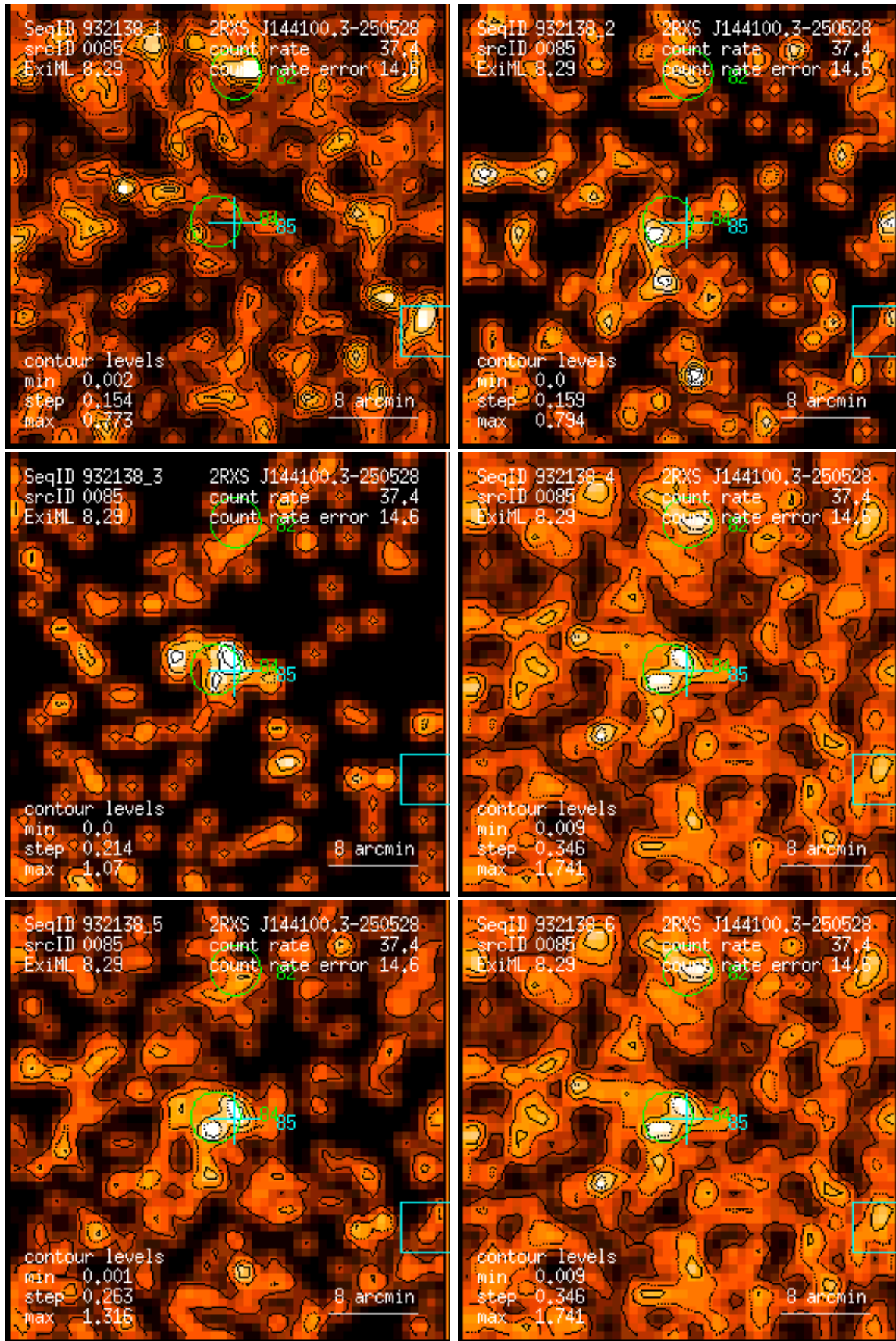
Figure 85: RASS 932138: detection 0085: band rate images, Gaussian filter: (1) PSPC channels 11 – 41, (2) 52 – 90, (3) 91 – 201, (4) 11 – 235, (5) 52 – 201, (6) 11 – 201. Broad band rates in counts/ks. Band rate contour levels in counts/ks/arcmin 2 .
