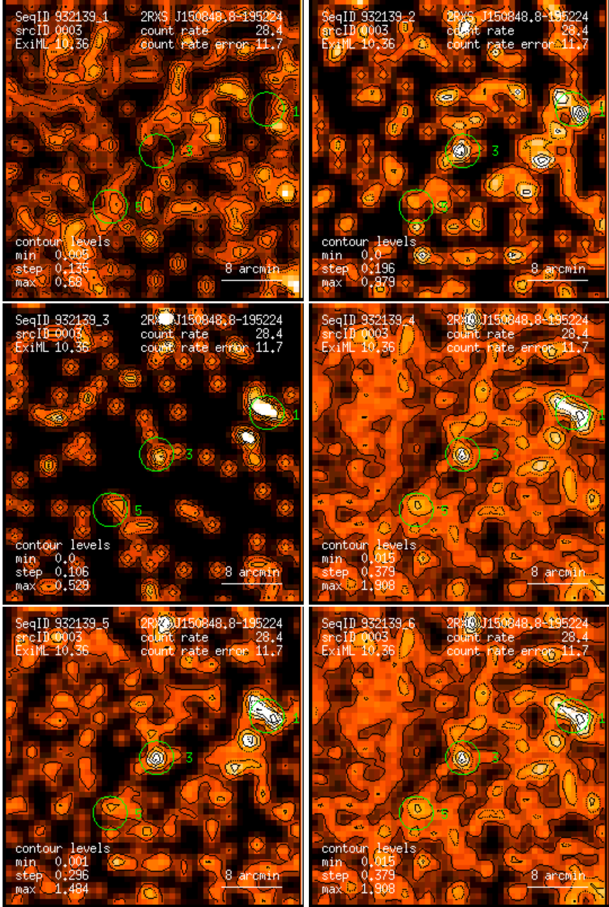
Figure 3: RASS 932139: detection 0003: band rate images, Gaussian filter: (1) PSPC channels 11 – 41, (2) 52 – 90, (3) 91 – 201, (4) 11 – 235, (5) 52 – 201, (6) 11 – 201. Broad band rates in counts/ks. Band rate contour levels in counts/ks/arcmin 2 .
