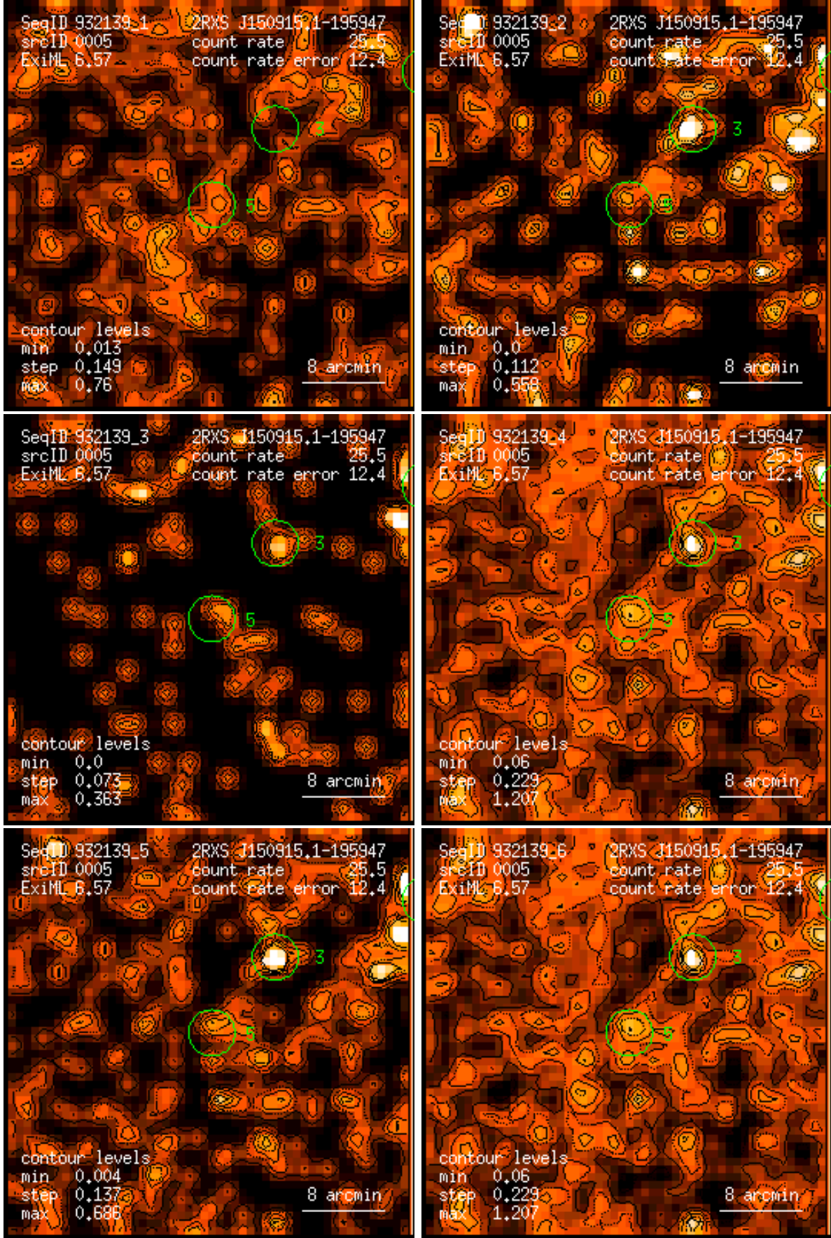
Figure 5: RASS 932139: detection 0005: band rate images, Gaussian filter: (1) PSPC channels 11 – 41, (2) 52 – 90, (3) 91 – 201, (4) 11 – 235, (5) 52 – 201, (6) 11 – 201. Broad band rates in counts/ks. Band rate contour levels in counts/ks/arcmin 2 .
