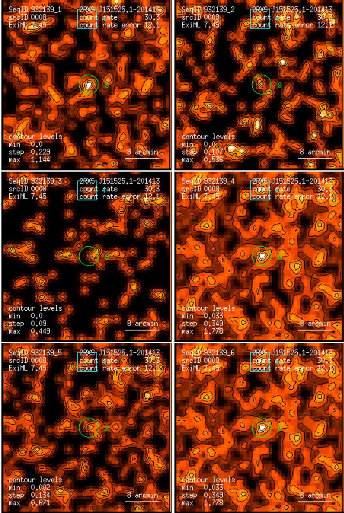
Figure 8: RASS 932139: detection 0008: band rate images, Gaussian filter: (1) PSPC channels 11 – 41, (2) 52 – 90, (3) 91 – 201, (4) 11 – 235, (5) 52 – 201, (6) 11 – 201. Broad band rates in counts/ks. Band rate contour levels in counts/ks/arcmin 2 .
