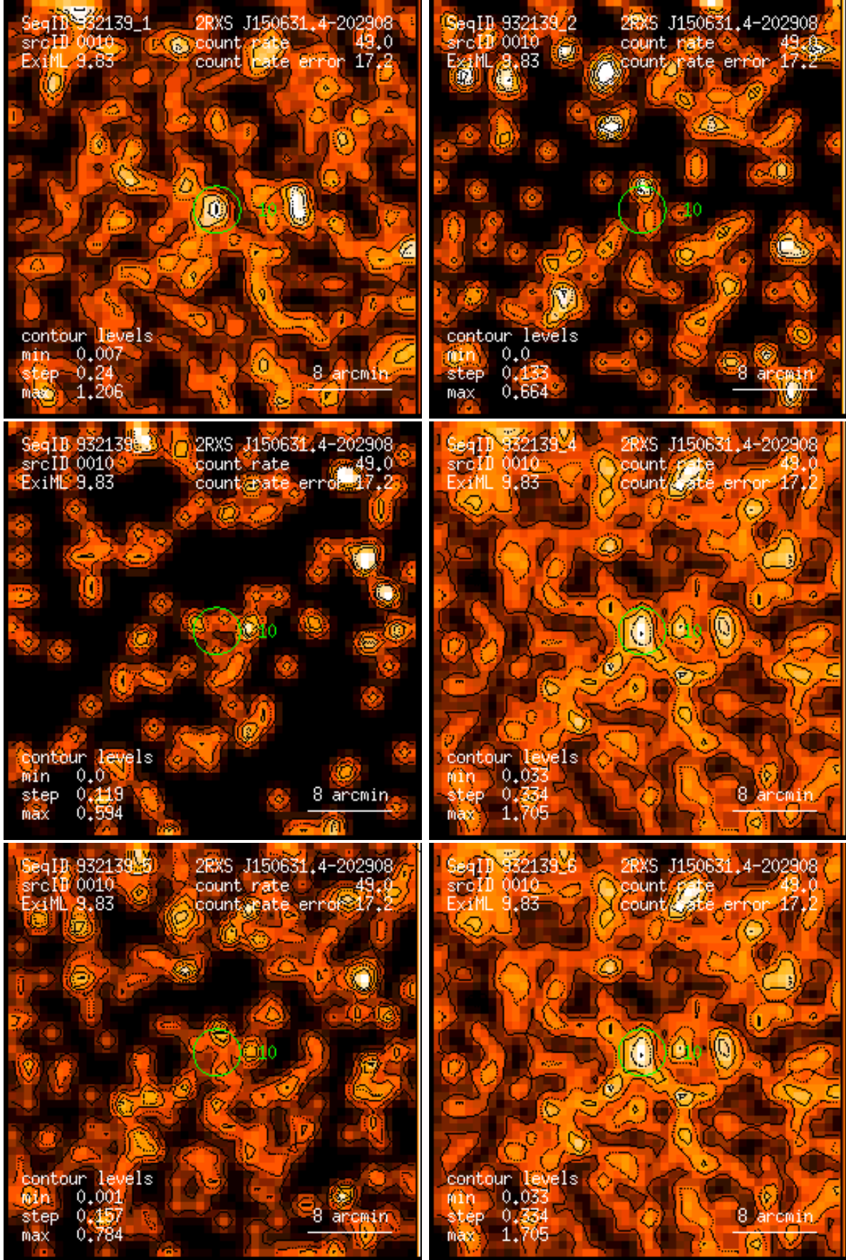
Figure 10: RASS 932139: detection 0010: band rate images, Gaussian filter: (1) PSPC channels 11 – 41, (2) 52 – 90, (3) 91 – 201, (4) 11 – 235, (5) 52 – 201, (6) 11 – 201. Broad band rates in counts/ks. Band rate contour levels in counts/ks/arcmin 2 .
