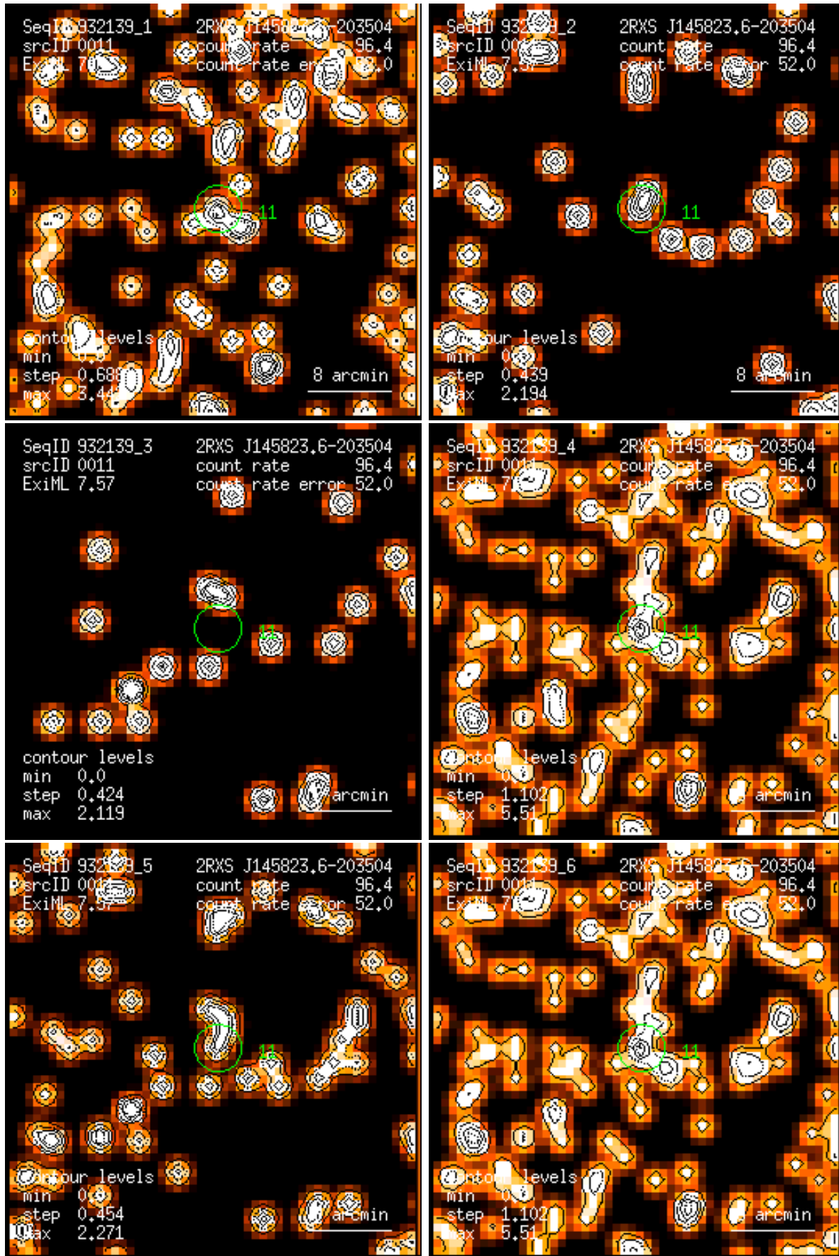
Figure 11: RASS 932139: detection 0011: band rate images, Gaussian filter: (1) PSPC channels 11 – 41, (2) 52 – 90, (3) 91 – 201, (4) 11 – 235, (5) 52 – 201, (6) 11 – 201. Broad band rates in counts/ks. Band rate contour levels in counts/ks/arcmin 2 .
