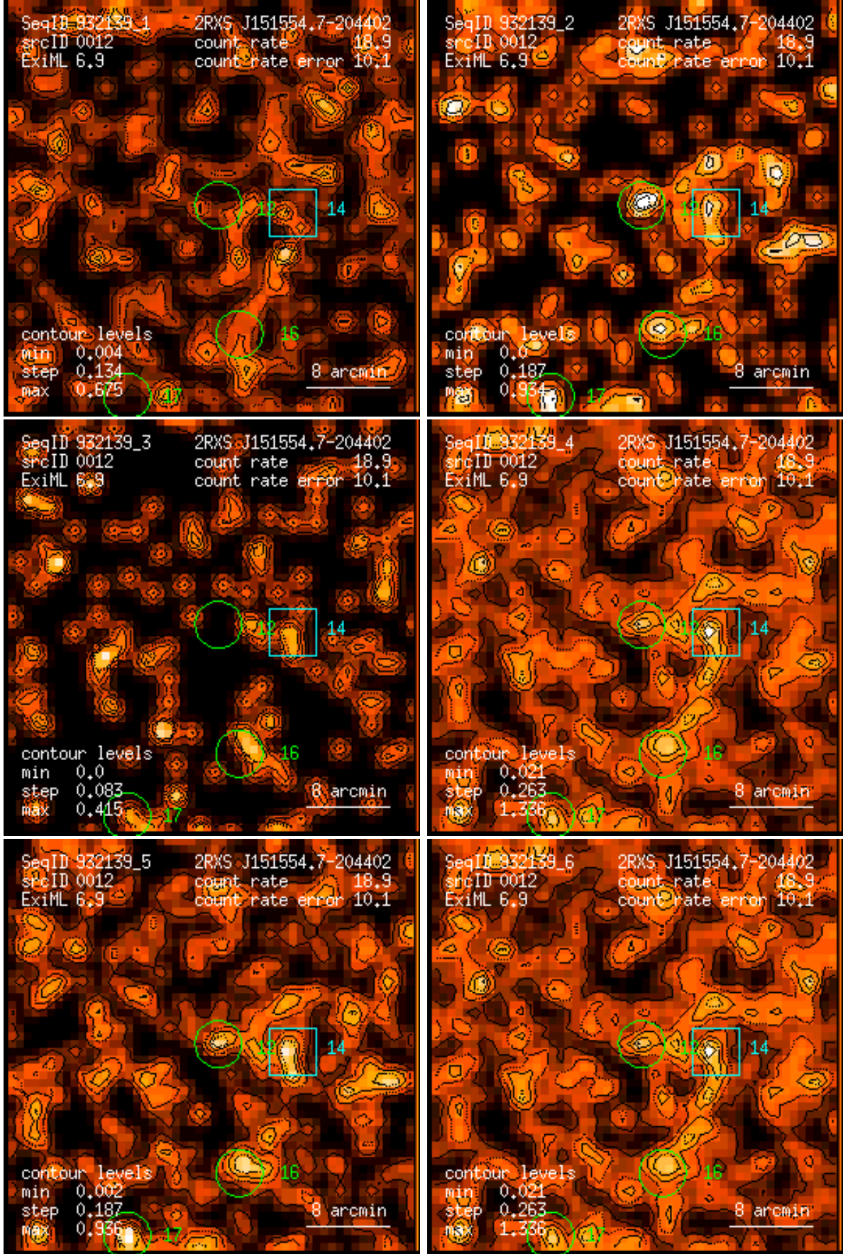
Figure 12: RASS 932139: detection 0012: band rate images, Gaussian filter: (1) PSPC channels 11 – 41, (2) 52 – 90, (3) 91 – 201, (4) 11 – 235, (5) 52 – 201, (6) 11 – 201. Broad band rates in counts/ks. Band rate contour levels in counts/ks/arcmin 2 .
