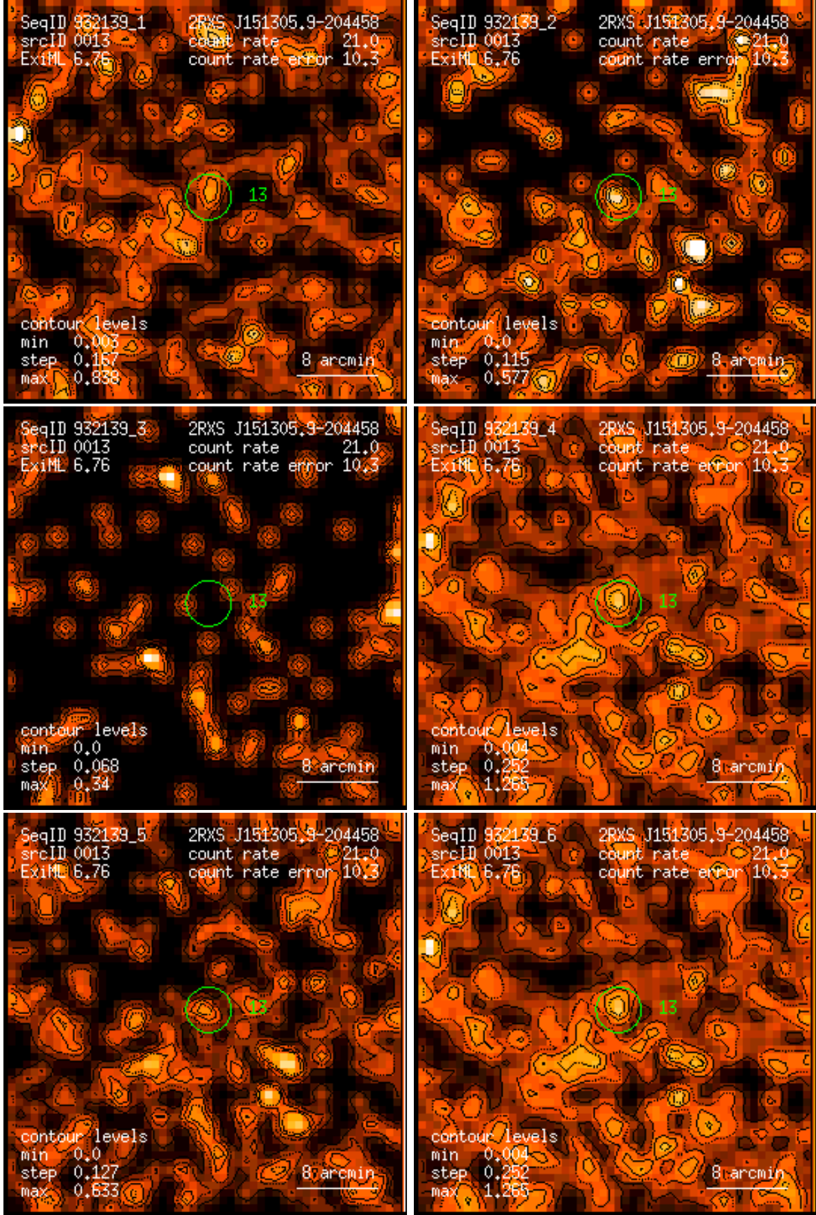
Figure 13: RASS 932139: detection 0013: band rate images, Gaussian filter: (1) PSPC channels 11 – 41, (2) 52 – 90, (3) 91 – 201, (4) 11 – 235, (5) 52 – 201, (6) 11 – 201. Broad band rates in counts/ks. Band rate contour levels in counts/ks/arcmin 2 .
