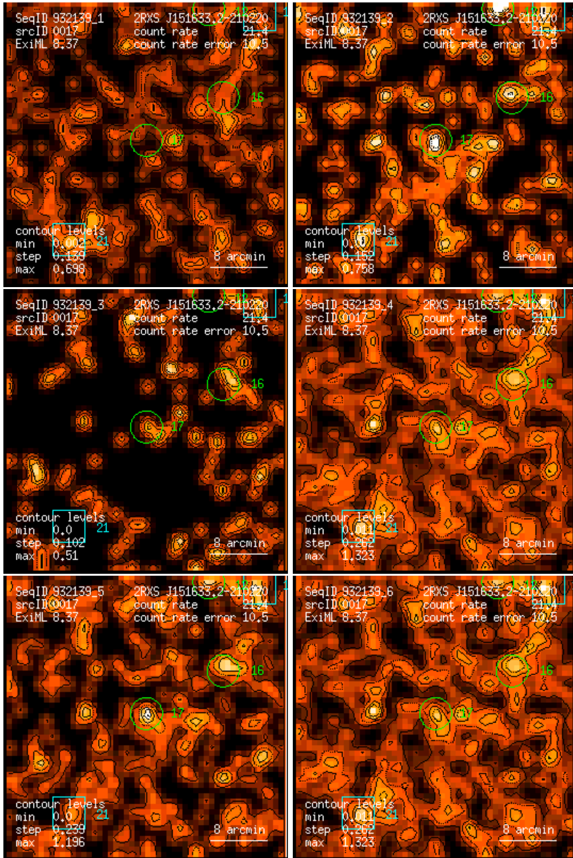
Figure 17: RASS 932139: detection 0017: band rate images, Gaussian filter: (1) PSPC channels 11 – 41, (2) 52 – 90, (3) 91 – 201, (4) 11 – 235, (5) 52 – 201, (6) 11 – 201. Broad band rates in counts/ks. Band rate contour levels in counts/ks/arcmin 2 .
