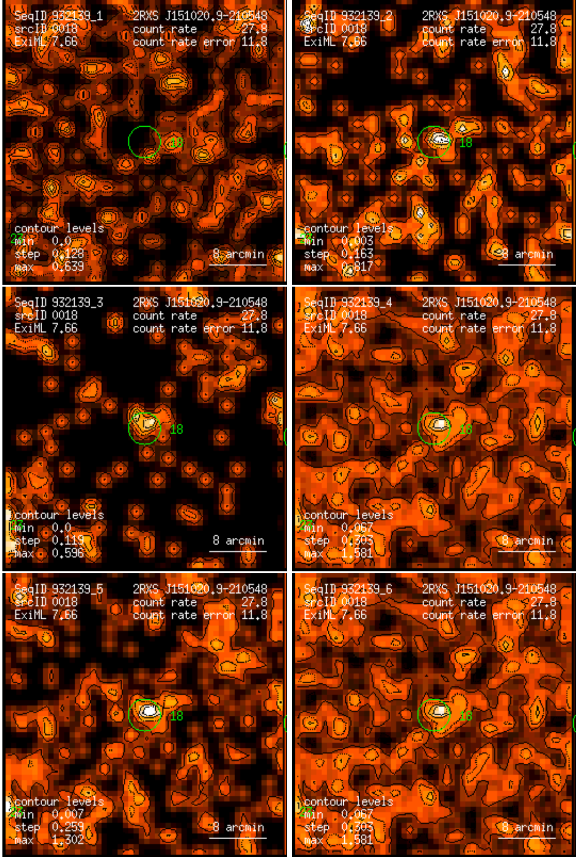
Figure 18: RASS 932139: detection 0018: band rate images, Gaussian filter: (1) PSPC channels 11 – 41, (2) 52 – 90, (3) 91 – 201, (4) 11 – 235, (5) 52 – 201, (6) 11 – 201. Broad band rates in counts/ks. Band rate contour levels in counts/ks/arcmin 2 .
