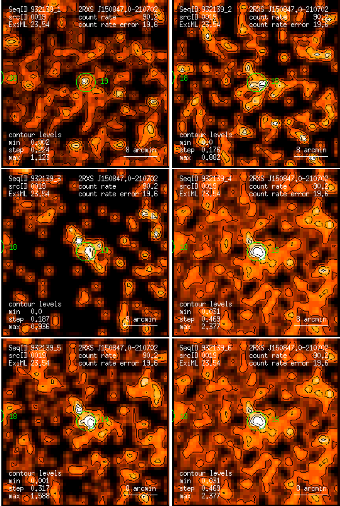
Figure 19: RASS 932139: detection 0019: band rate images, Gaussian filter: (1) PSPC channels 11 – 41, (2) 52 – 90, (3) 91 – 201, (4) 11 – 235, (5) 52 – 201, (6) 11 – 201. Broad band rates in counts/ks. Band rate contour levels in counts/ks/arcmin 2 .
