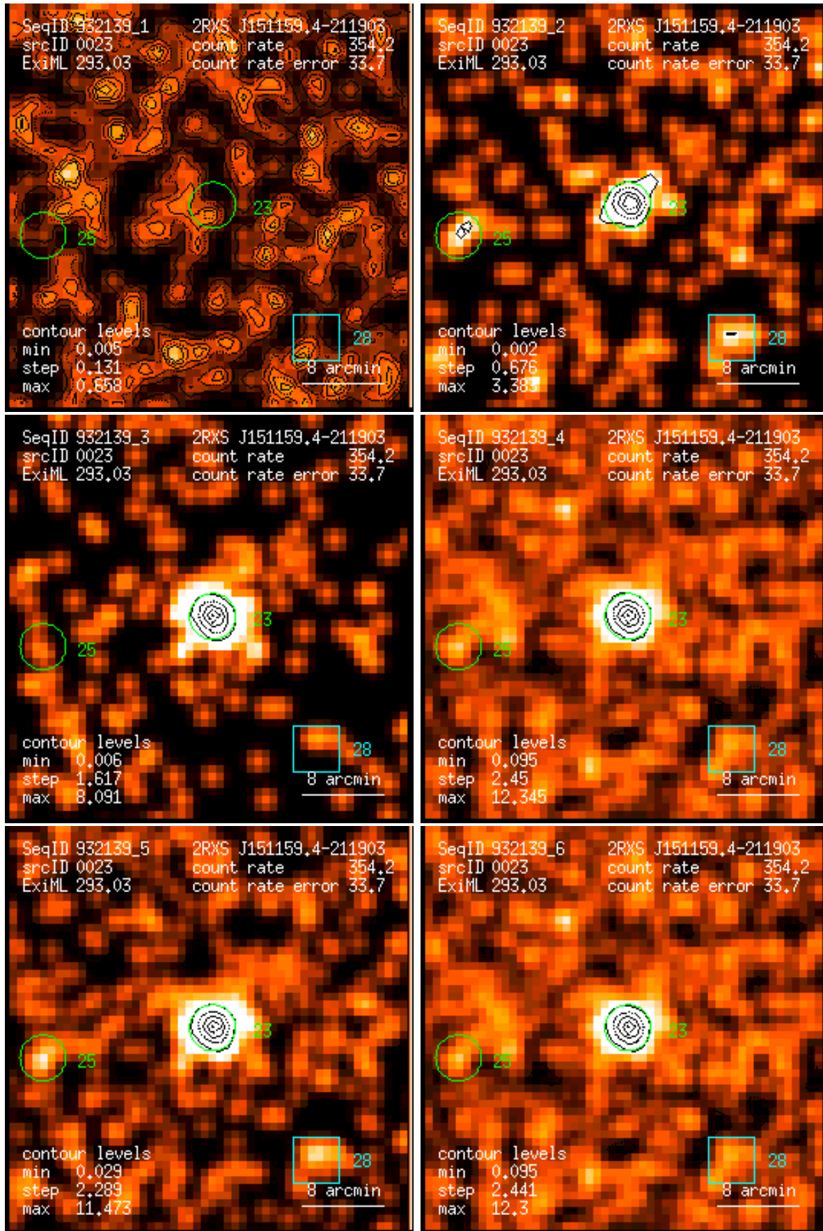
Figure 23: RASS 932139: detection 0023: band rate images, Gaussian filter: (1) PSPC channels 11 – 41, (2) 52 – 90, (3) 91 – 201, (4) 11 – 235, (5) 52 – 201, (6) 11 – 201. Broad band rates in counts/ks. Band rate contour levels in counts/ks/arcmin 2 .
