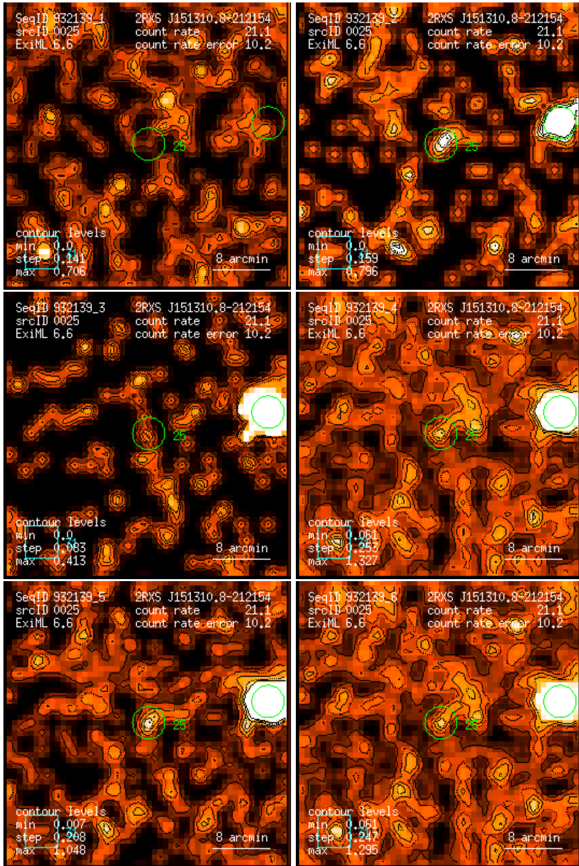
Figure 25: RASS 932139: detection 0025: band rate images, Gaussian filter: (1) PSPC channels 11 – 41, (2) 52 – 90, (3) 91 – 201, (4) 11 – 235, (5) 52 – 201, (6) 11 – 201. Broad band rates in counts/ks. Band rate contour levels in counts/ks/arcmin 2 .
