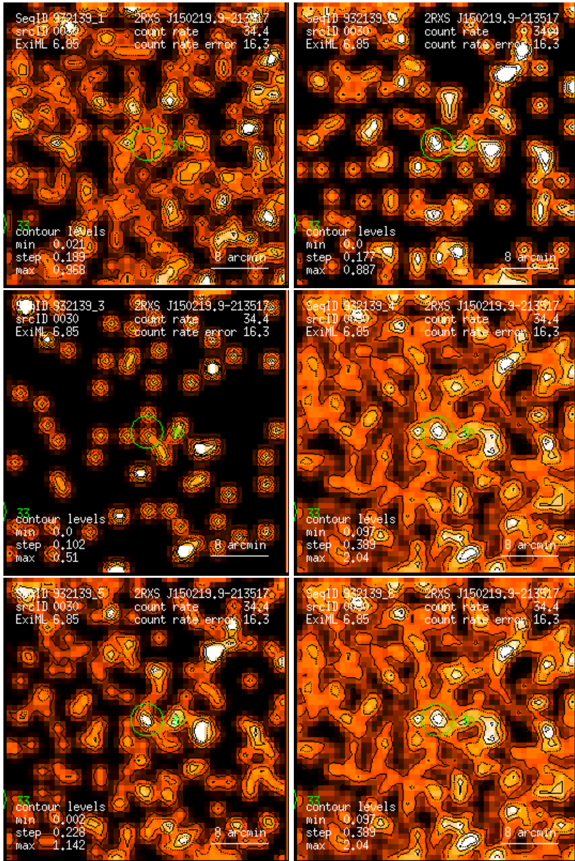
Figure 30: RASS 932139: detection 0030: band rate images, Gaussian filter: (1) PSPC channels 11 – 41, (2) 52 – 90, (3) 91 – 201, (4) 11 – 235, (5) 52 – 201, (6) 11 – 201. Broad band rates in counts/ks. Band rate contour levels in counts/ks/arcmin 2 .
