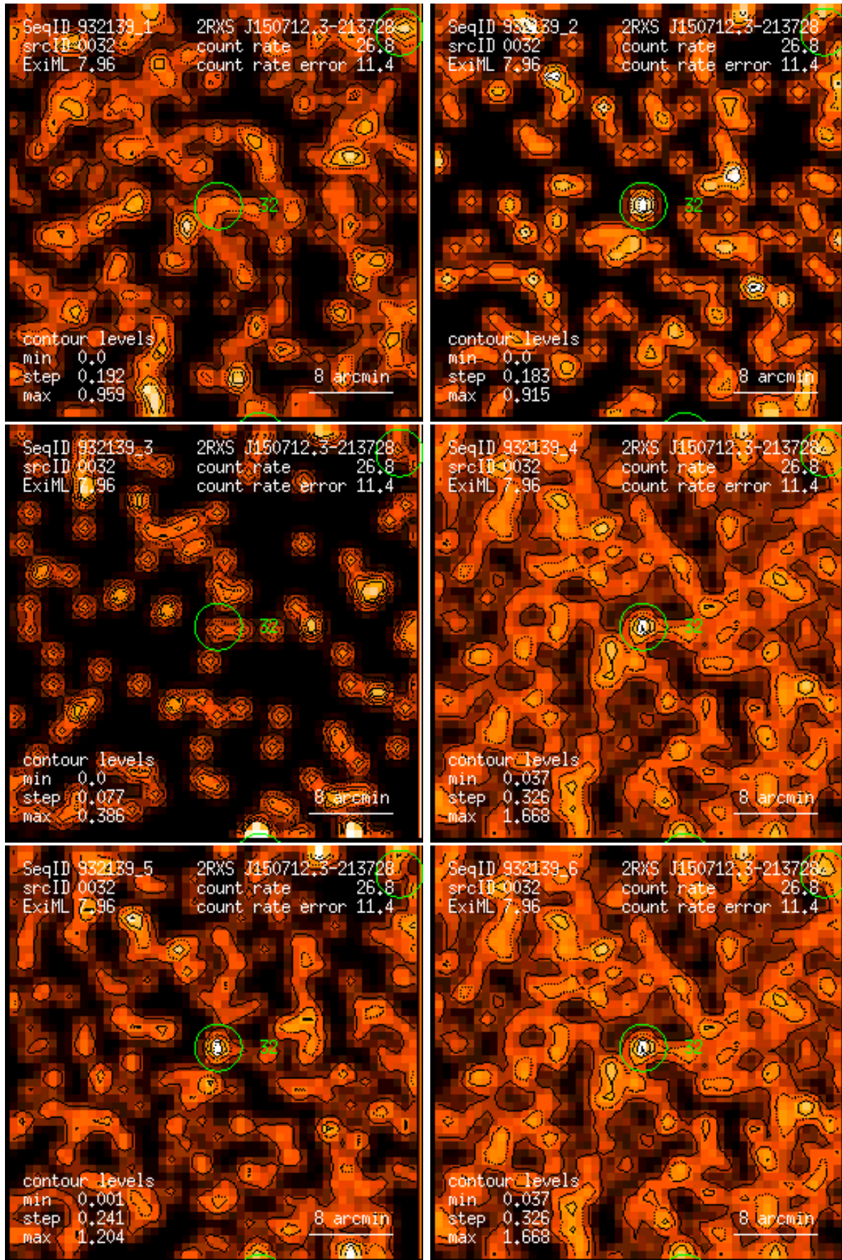
Figure 32: RASS 932139: detection 0032: band rate images, Gaussian filter: (1) PSPC channels 11 – 41, (2) 52 – 90, (3) 91 – 201, (4) 11 – 235, (5) 52 – 201, (6) 11 – 201. Broad band rates in counts/ks. Band rate contour levels in counts/ks/arcmin 2 .
