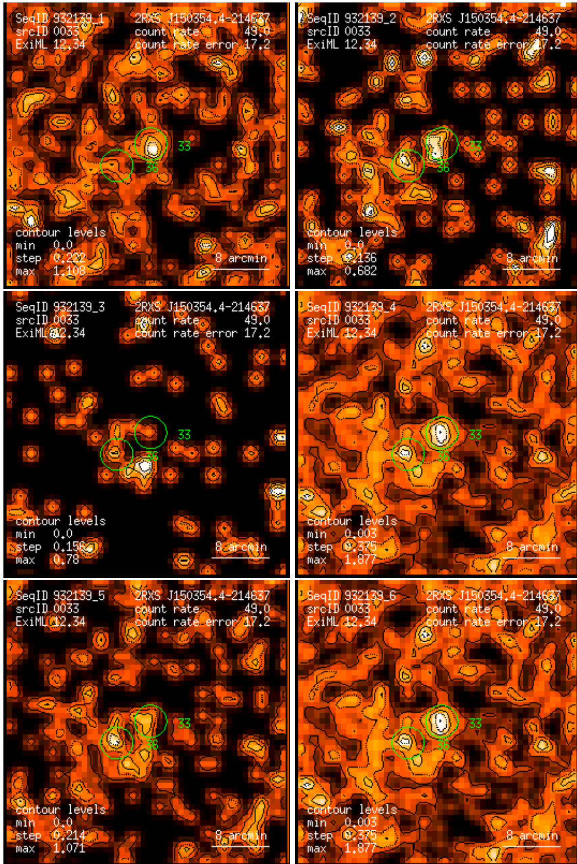
Figure 33: RASS 932139: detection 0033: band rate images, Gaussian filter: (1) PSPC channels 11 – 41, (2) 52 – 90, (3) 91 – 201, (4) 11 – 235, (5) 52 – 201, (6) 11 – 201. Broad band rates in counts/ks. Band rate contour levels in counts/ks/arcmin 2 .
