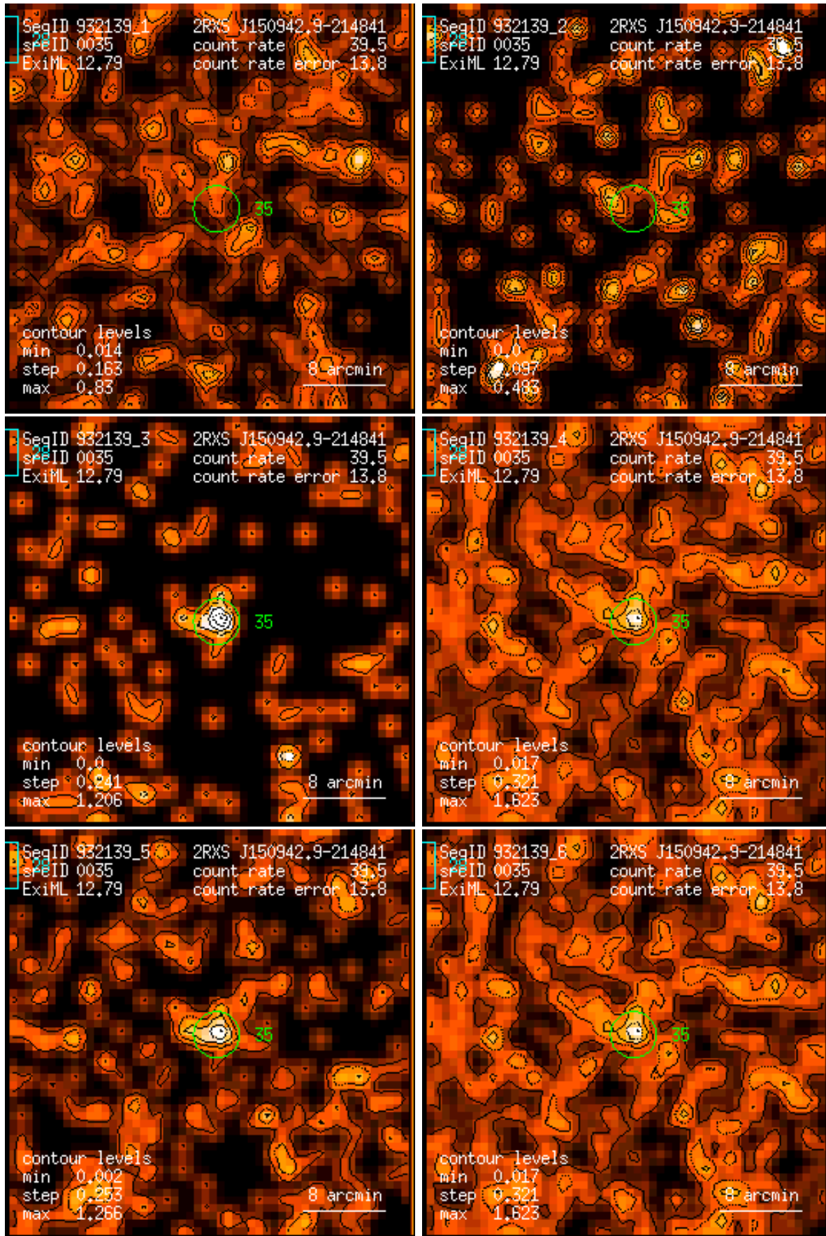
Figure 35: RASS 932139: detection 0035: band rate images, Gaussian filter: (1) PSPC channels 11 – 41, (2) 52 – 90, (3) 91 – 201, (4) 11 – 235, (5) 52 – 201, (6) 11 – 201. Broad band rates in counts/ks. Band rate contour levels in counts/ks/arcmin 2 .
