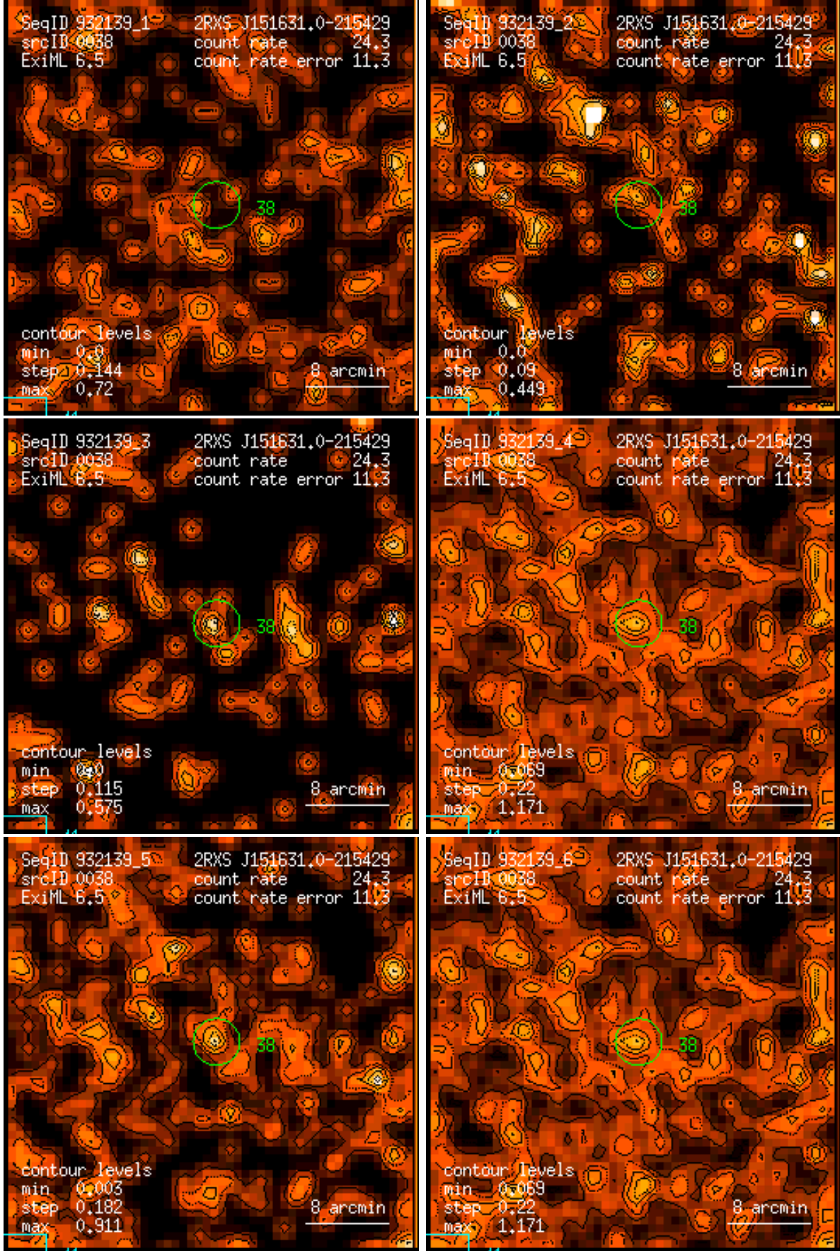
Figure 38: RASS 932139: detection 0038: band rate images, Gaussian filter: (1) PSPC channels 11 – 41, (2) 52 – 90, (3) 91 – 201, (4) 11 – 235, (5) 52 – 201, (6) 11 – 201. Broad band rates in counts/ks. Band rate contour levels in counts/ks/arcmin 2 .
