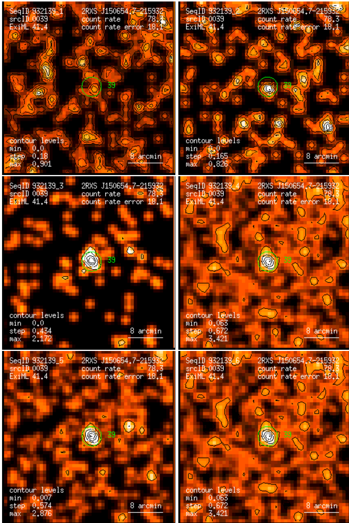
Figure 39: RASS 932139: detection 0039: band rate images, Gaussian filter: (1) PSPC channels 11 – 41, (2) 52 – 90, (3) 91 – 201, (4) 11 – 235, (5) 52 – 201, (6) 11 – 201. Broad band rates in counts/ks. Band rate contour levels in counts/ks/arcmin 2 .
