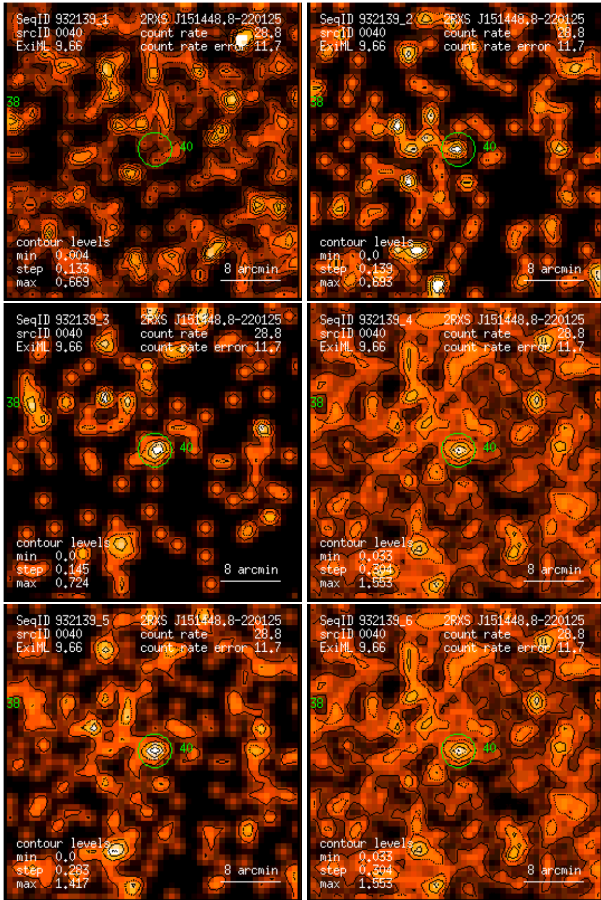
Figure 40: RASS 932139: detection 0040: band rate images, Gaussian filter: (1) PSPC channels 11 – 41, (2) 52 – 90, (3) 91 – 201, (4) 11 – 235, (5) 52 – 201, (6) 11 – 201. Broad band rates in counts/ks. Band rate contour levels in counts/ks/arcmin 2 .
