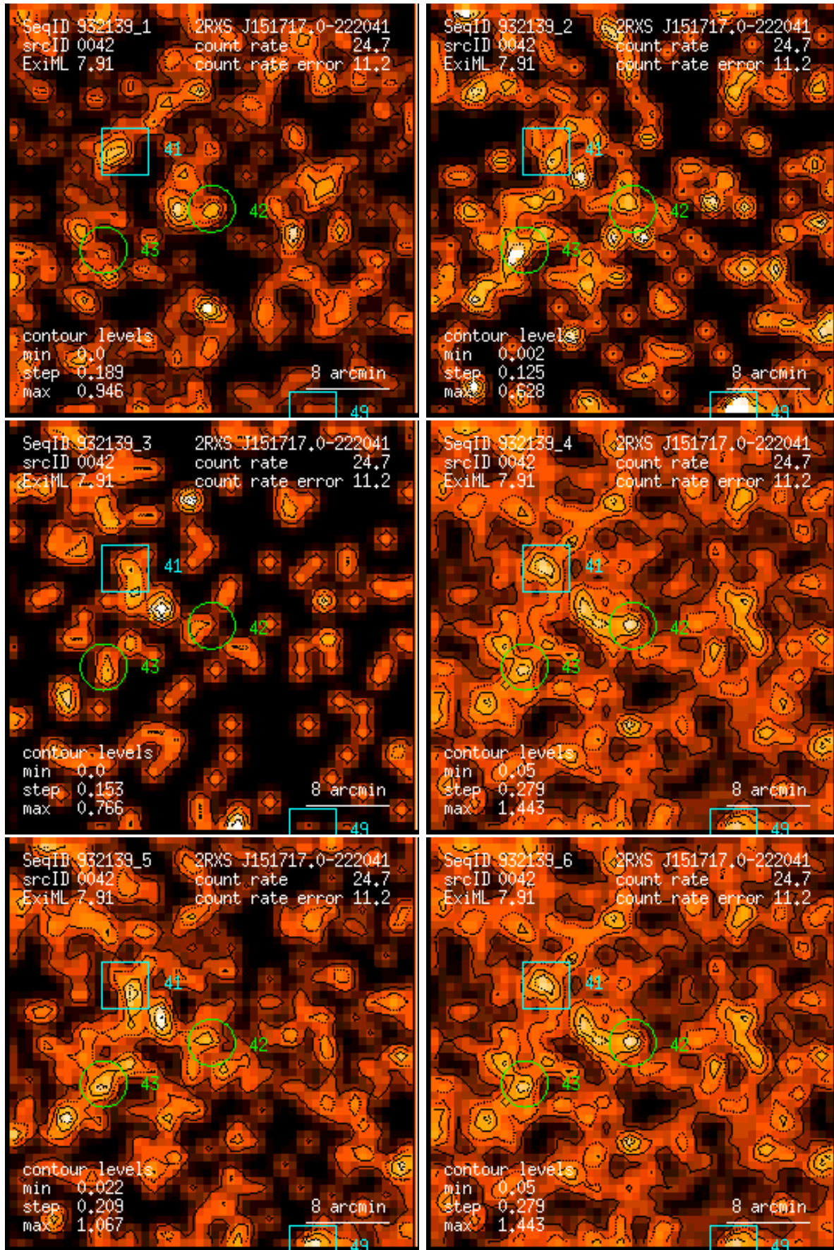
Figure 42: RASS 932139: detection 0042: band rate images, Gaussian filter: (1) PSPC channels 11 – 41, (2) 52 – 90, (3) 91 – 201, (4) 11 – 235, (5) 52 – 201, (6) 11 – 201. Broad band rates in counts/ks. Band rate contour levels in counts/ks/arcmin 2 .
