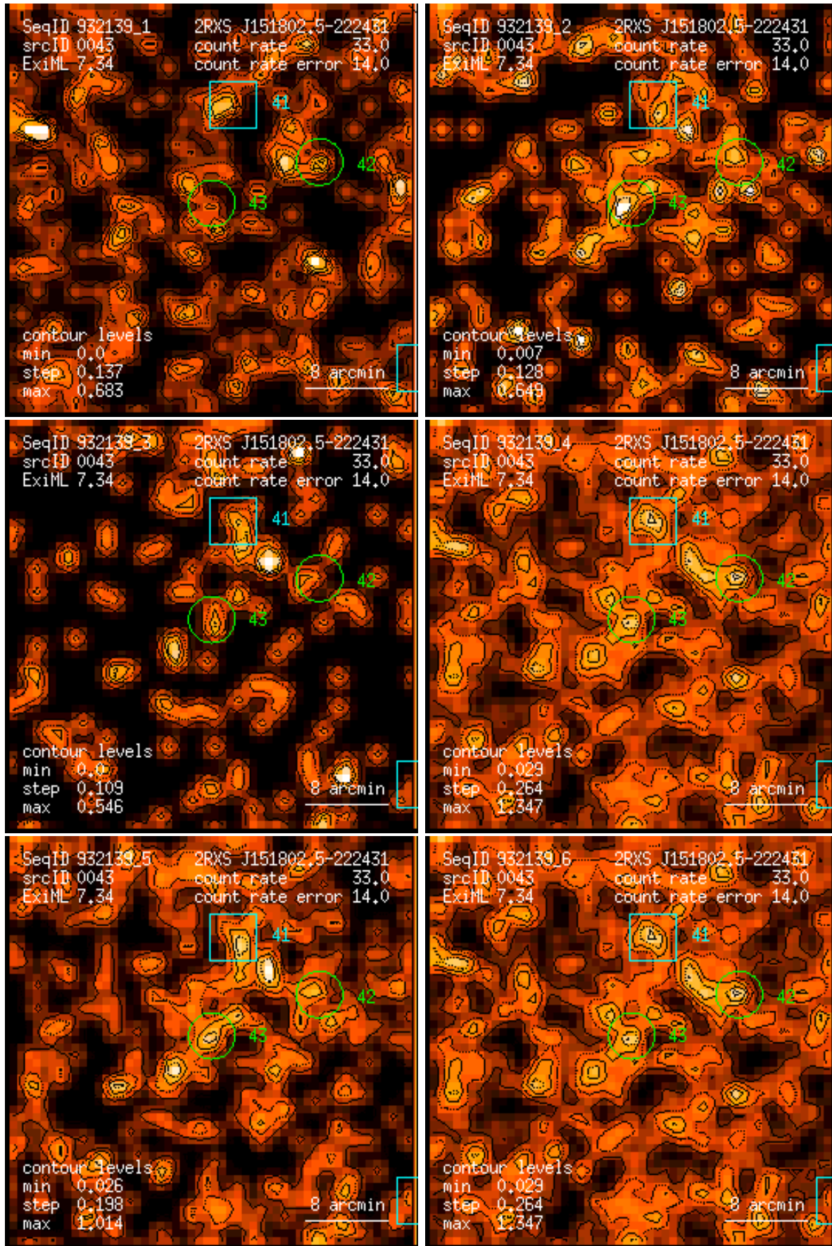
Figure 43: RASS 932139: detection 0043: band rate images, Gaussian filter: (1) PSPC channels 11 – 41, (2) 52 – 90, (3) 91 – 201, (4) 11 – 235, (5) 52 – 201, (6) 11 – 201. Broad band rates in counts/ks. Band rate contour levels in counts/ks/arcmin 2 .
