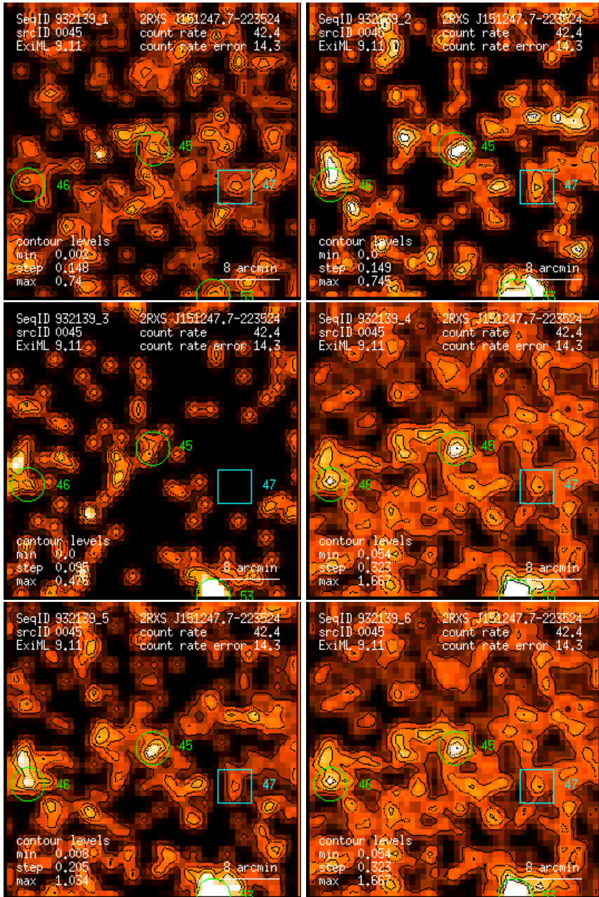
Figure 45: RASS 932139: detection 0045: band rate images, Gaussian filter: (1) PSPC channels 11 – 41, (2) 52 – 90, (3) 91 – 201, (4) 11 – 235, (5) 52 – 201, (6) 11 – 201. Broad band rates in counts/ks. Band rate contour levels in counts/ks/arcmin 2 .
