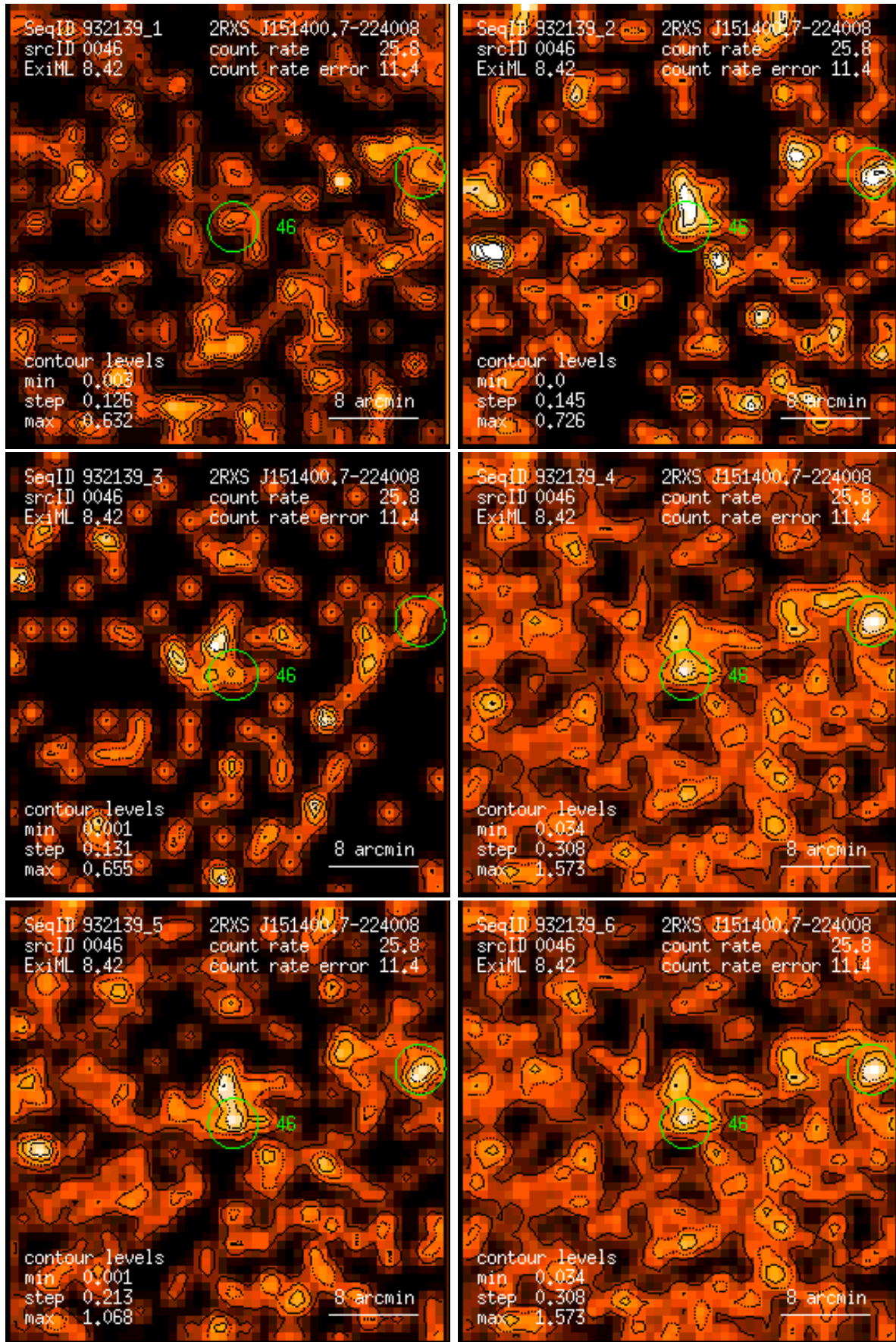
Figure 46: RASS 932139: detection 0046: band rate images, Gaussian filter: (1) PSPC channels 11 – 41, (2) 52 – 90, (3) 91 – 201, (4) 11 – 235, (5) 52 – 201, (6) 11 – 201. Broad band rates in counts/ks. Band rate contour levels in counts/ks/arcmin 2 .
