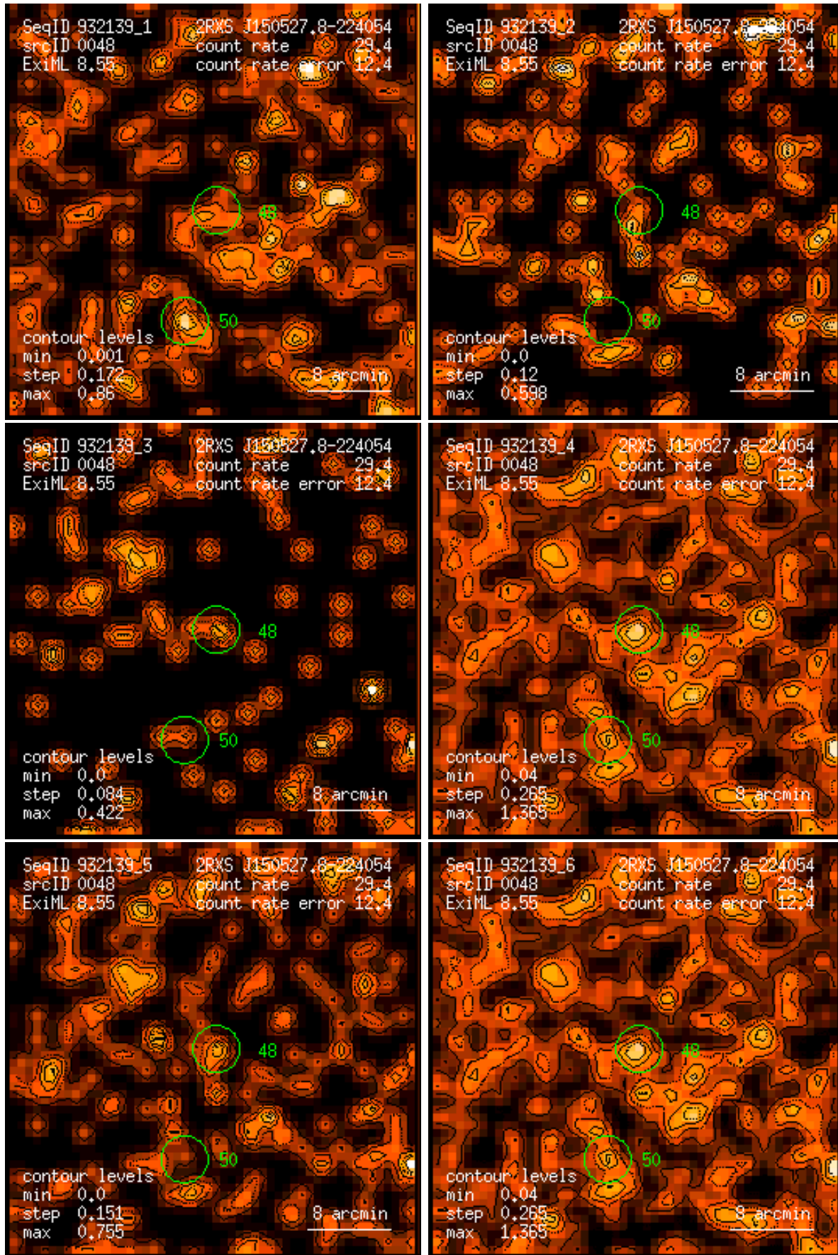
Figure 48: RASS 932139: detection 0048: band rate images, Gaussian filter: (1) PSPC channels 11 – 41, (2) 52 – 90, (3) 91 – 201, (4) 11 – 235, (5) 52 – 201, (6) 11 – 201. Broad band rates in counts/ks. Band rate contour levels in counts/ks/arcmin 2 .
