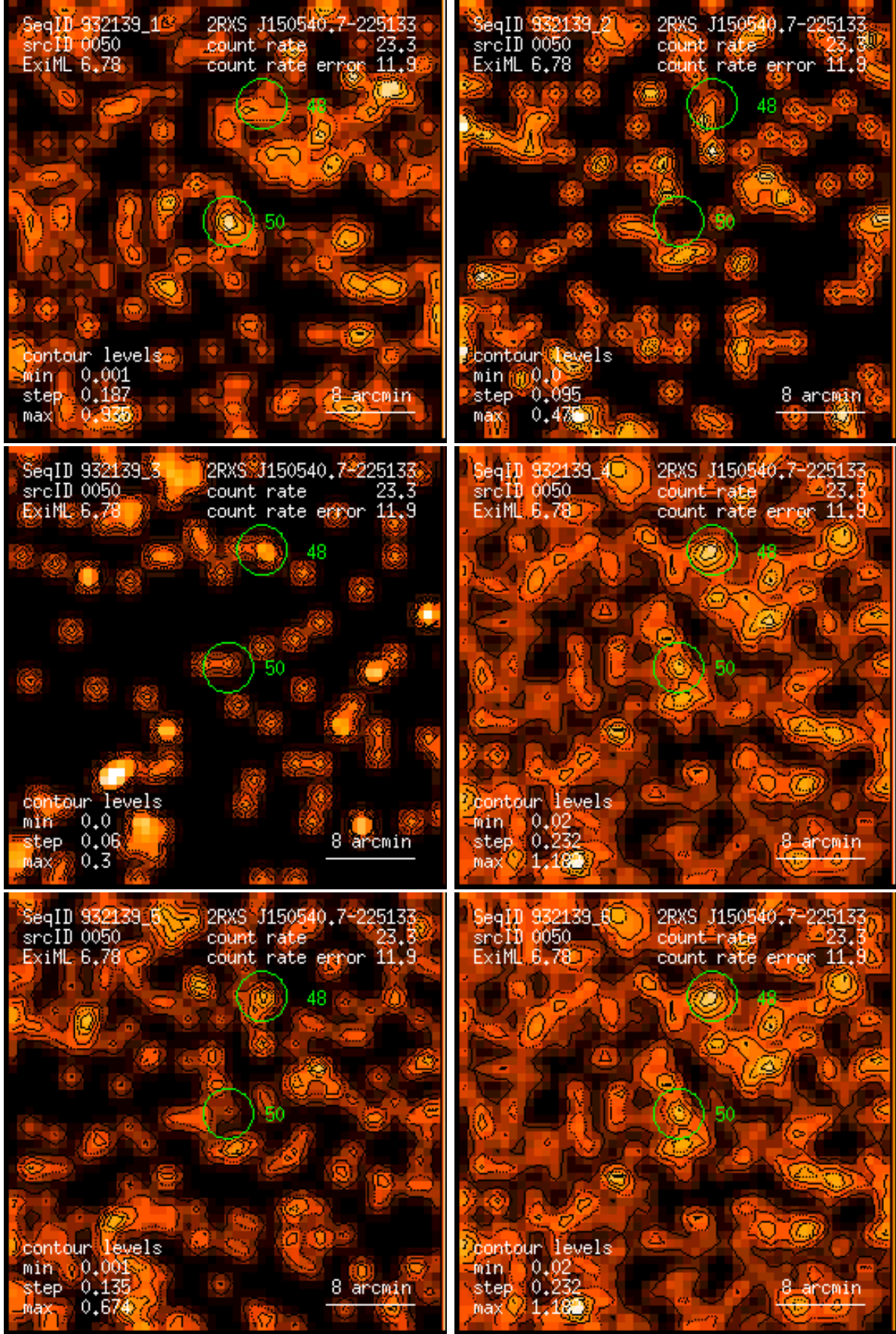
Figure 50: RASS 932139: detection 0050: band rate images, Gaussian filter: (1) PSPC channels 11 – 41, (2) 52 – 90, (3) 91 – 201, (4) 11 – 235, (5) 52 – 201, (6) 11 – 201. Broad band rates in counts/ks. Band rate contour levels in counts/ks/arcmin 2 .
