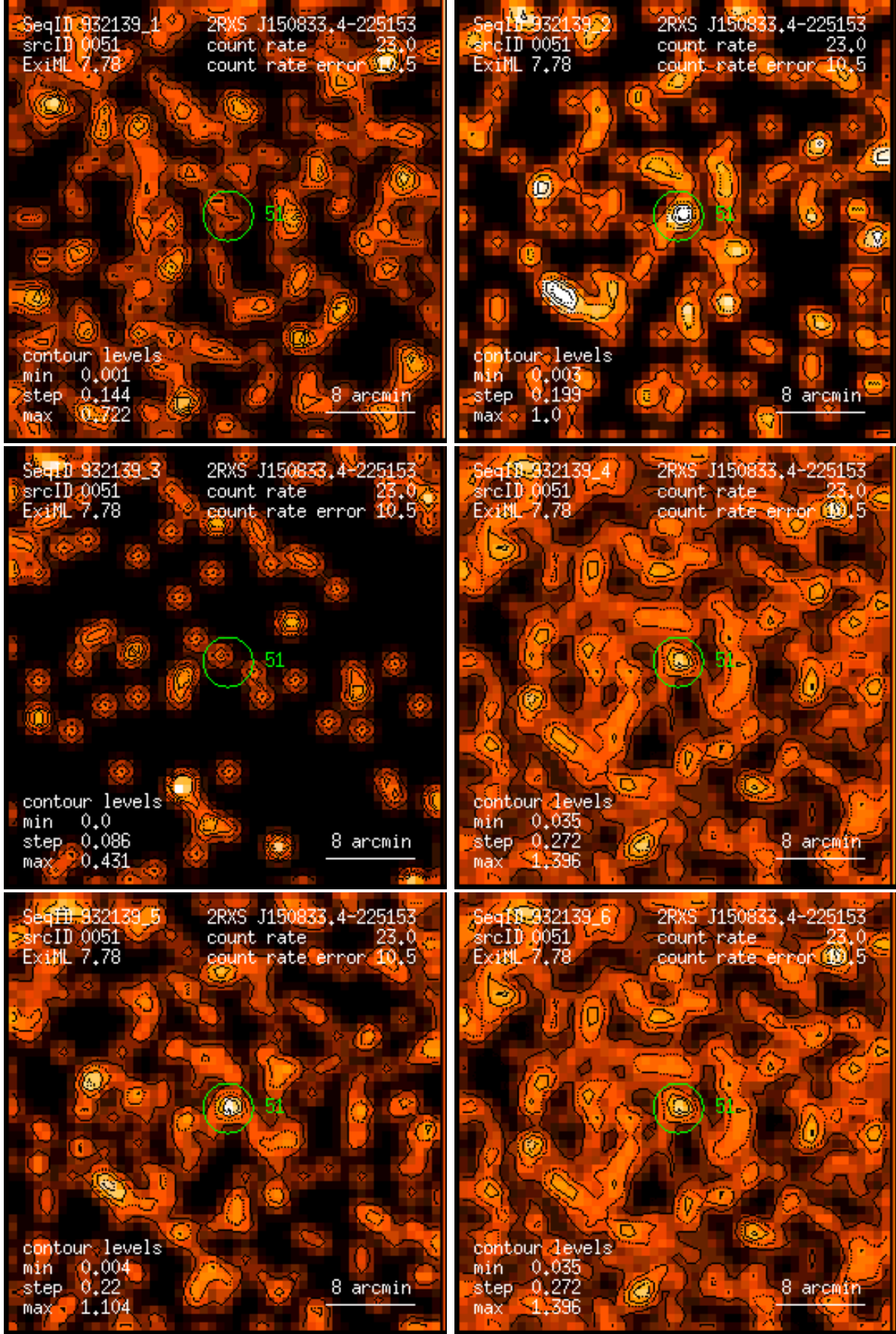
Figure 51: RASS 932139: detection 0051: band rate images, Gaussian filter: (1) PSPC channels 11 – 41, (2) 52 – 90, (3) 91 – 201, (4) 11 – 235, (5) 52 – 201, (6) 11 – 201. Broad band rates in counts/ks. Band rate contour levels in counts/ks/arcmin 2 .
