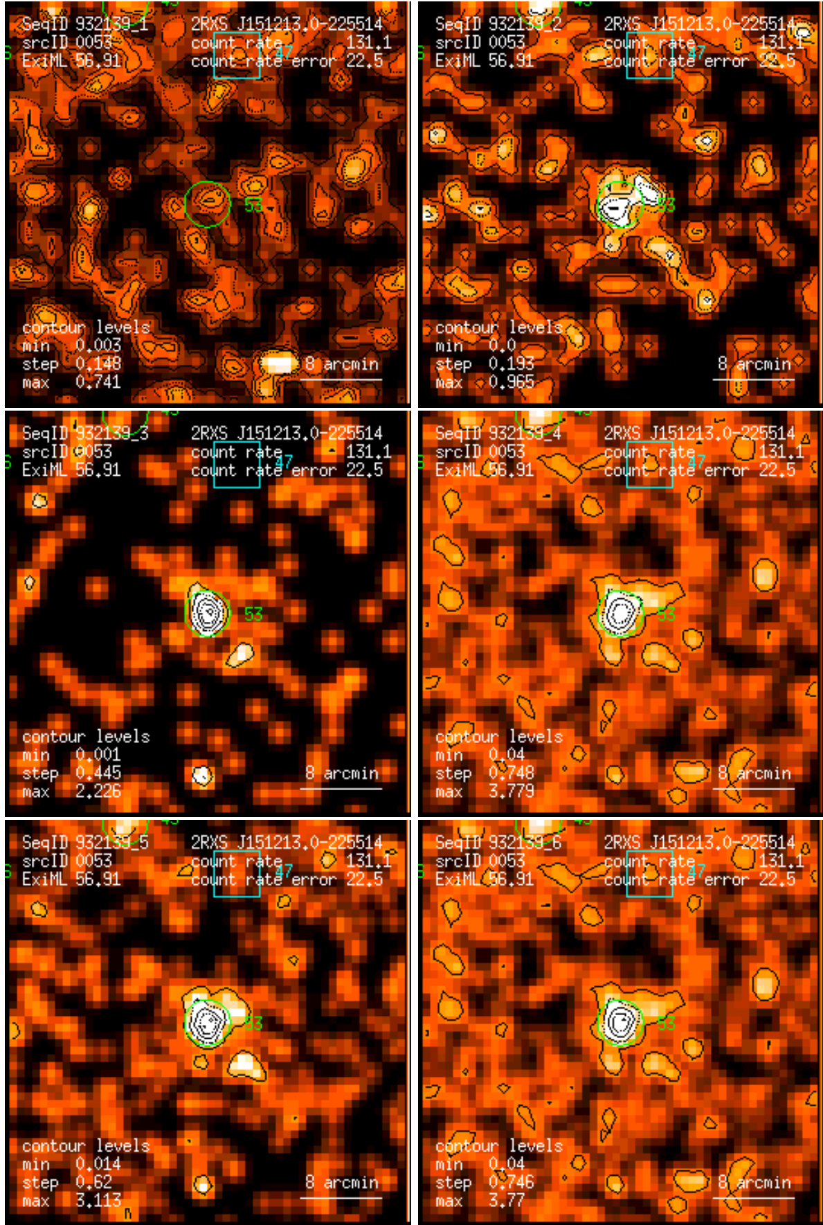
Figure 53: RASS 932139: detection 0053: band rate images, Gaussian filter: (1) PSPC channels 11 – 41, (2) 52 – 90, (3) 91 – 201, (4) 11 – 235, (5) 52 – 201, (6) 11 – 201. Broad band rates in counts/ks. Band rate contour levels in counts/ks/arcmin 2 .
