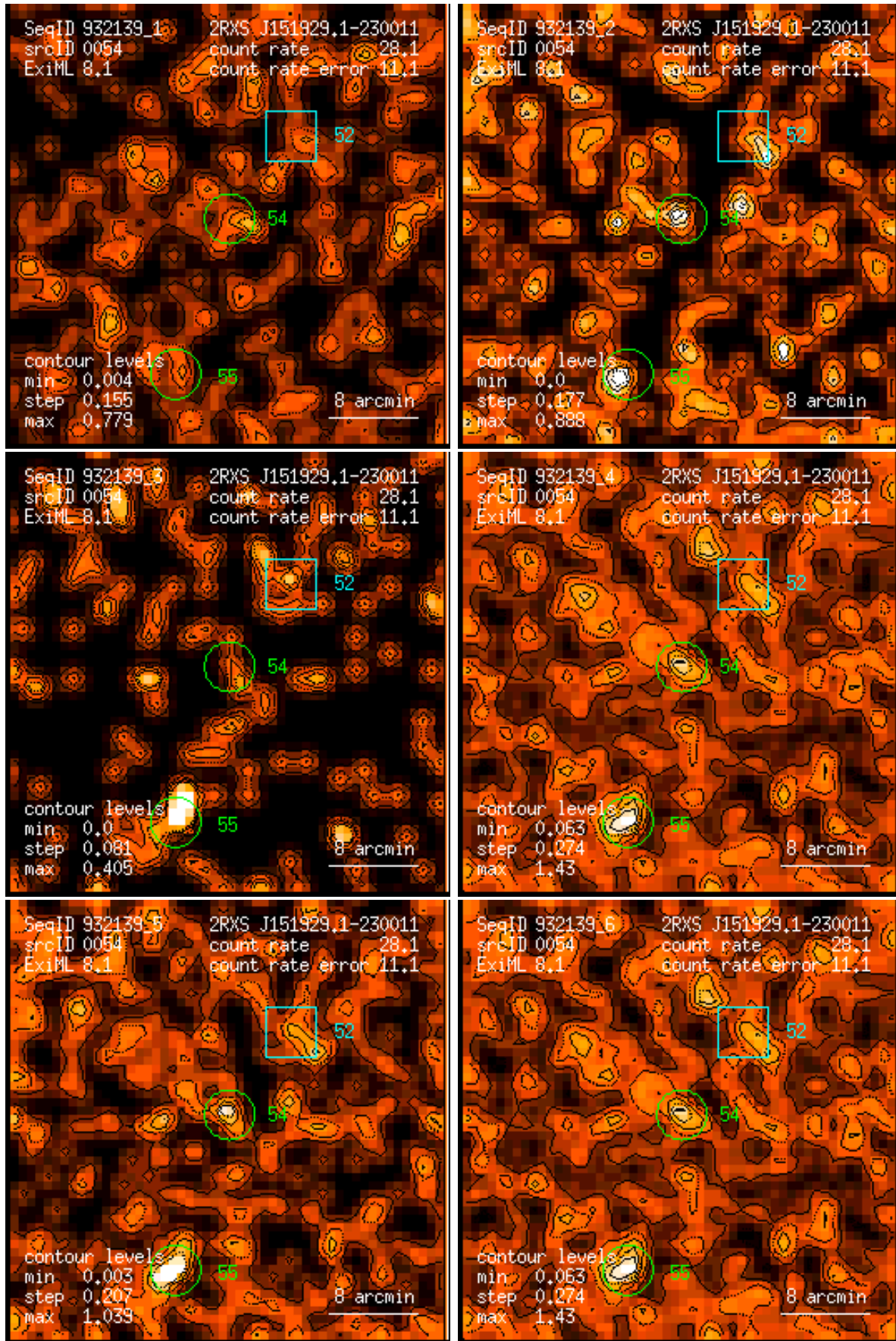
Figure 54: RASS 932139: detection 0054: band rate images, Gaussian filter: (1) PSPC channels 11 – 41, (2) 52 – 90, (3) 91 – 201, (4) 11 – 235, (5) 52 – 201, (6) 11 – 201. Broad band rates in counts/ks. Band rate contour levels in counts/ks/arcmin 2 .
