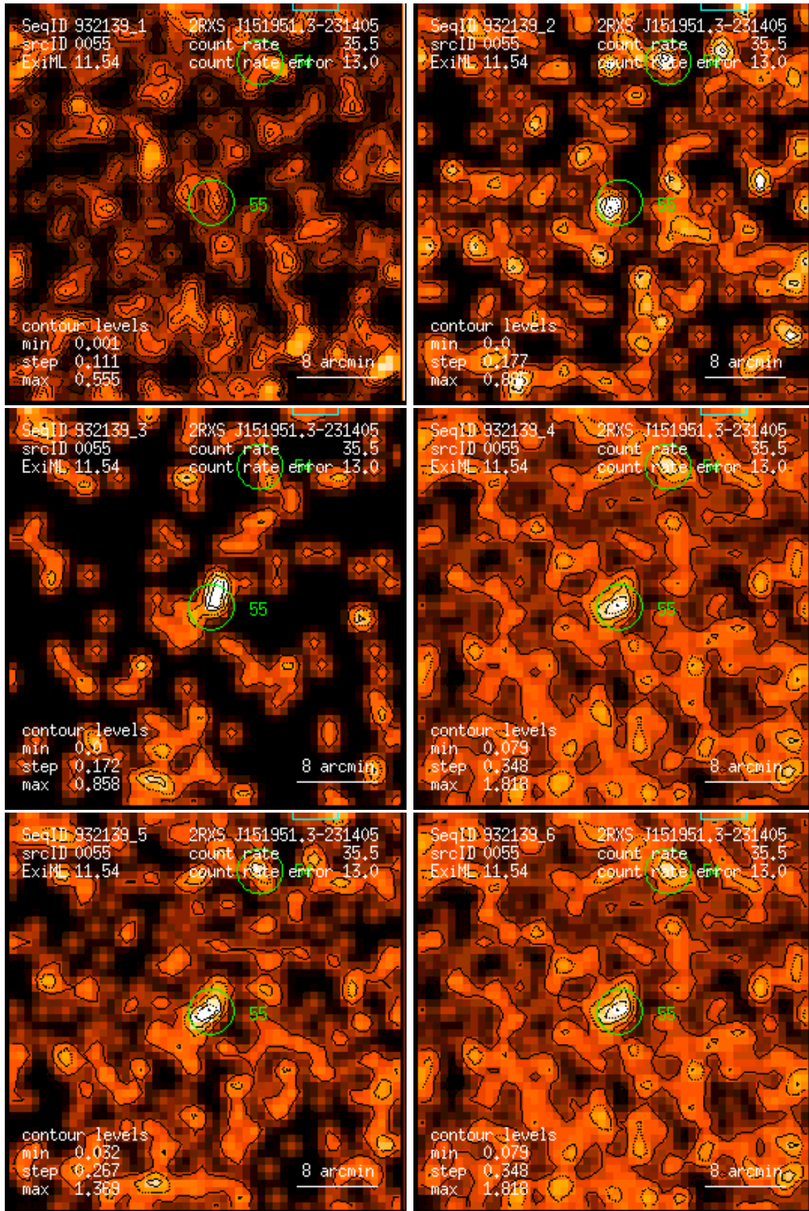
Figure 55: RASS 932139: detection 0055: band rate images, Gaussian filter: (1) PSPC channels 11 – 41, (2) 52 – 90, (3) 91 – 201, (4) 11 – 235, (5) 52 – 201, (6) 11 – 201. Broad band rates in counts/ks. Band rate contour levels in counts/ks/arcmin 2 .
