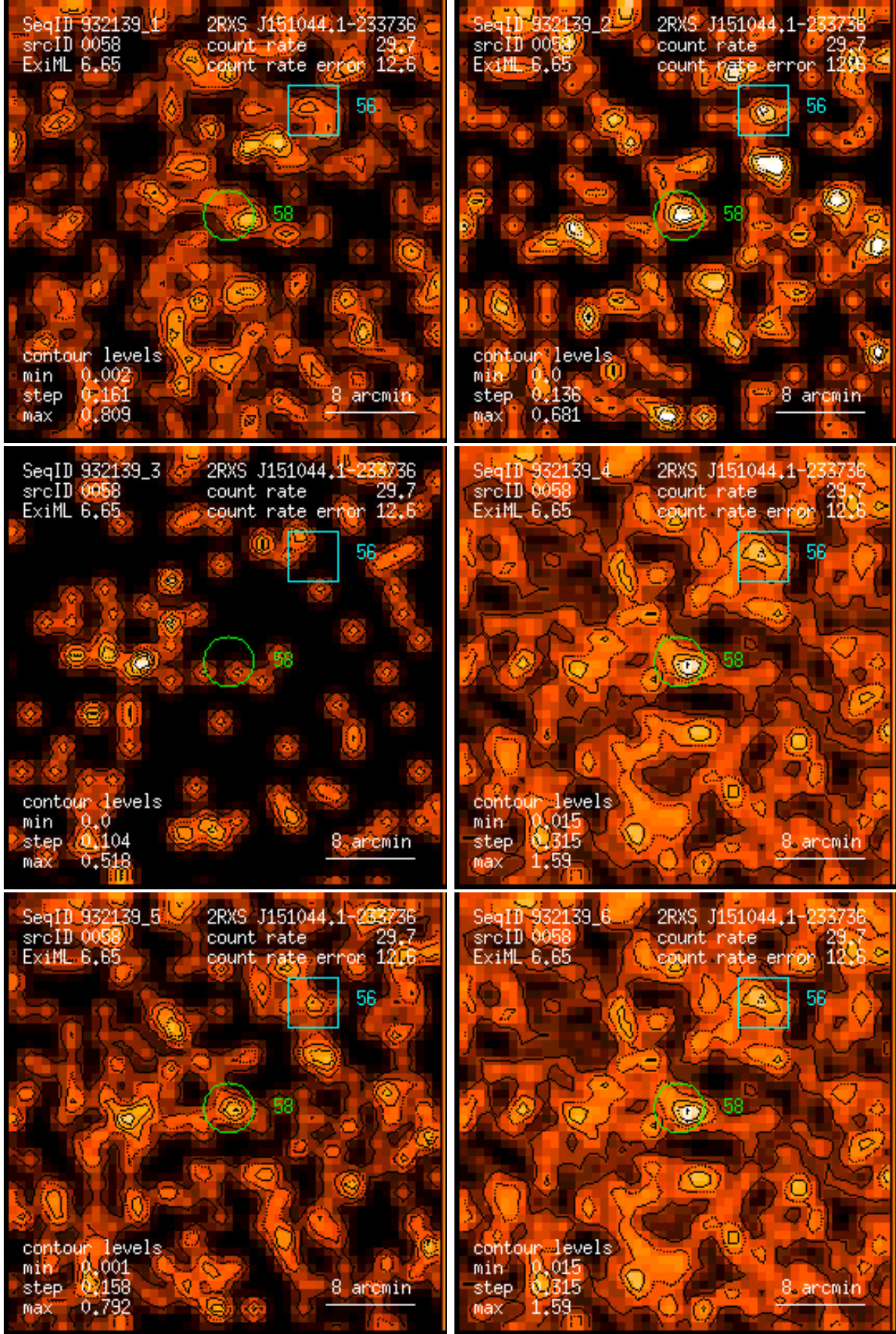
Figure 58: RASS 932139: detection 0058: band rate images, Gaussian filter: (1) PSPC channels 11 – 41, (2) 52 – 90, (3) 91 – 201, (4) 11 – 235, (5) 52 – 201, (6) 11 – 201. Broad band rates in counts/ks. Band rate contour levels in counts/ks/arcmin 2 .
