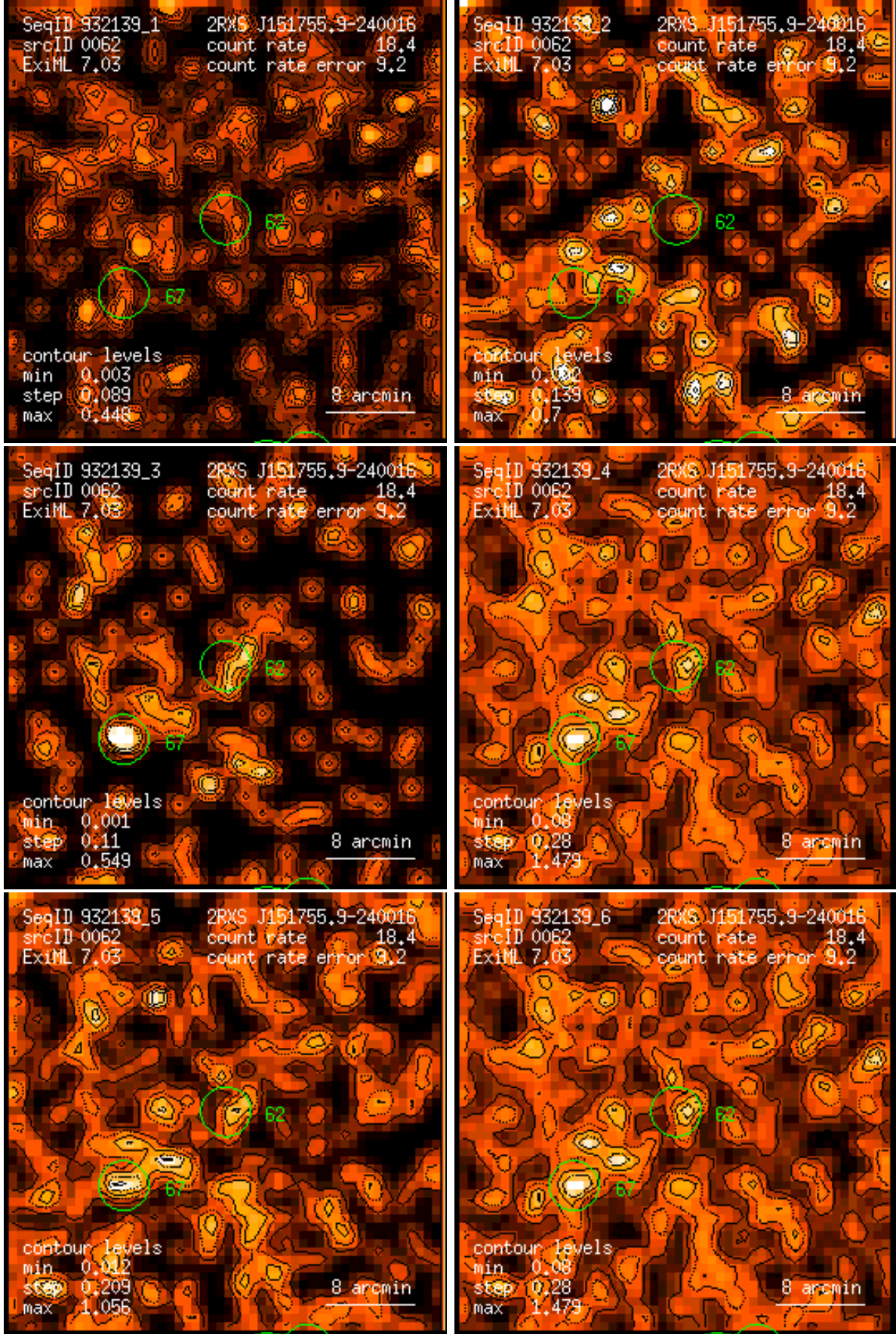
Figure 62: RASS 932139: detection 0062: band rate images, Gaussian filter: (1) PSPC channels 11 – 41, (2) 52 – 90, (3) 91 – 201, (4) 11 – 235, (5) 52 – 201, (6) 11 – 201. Broad band rates in counts/ks. Band rate contour levels in counts/ks/arcmin 2 .
