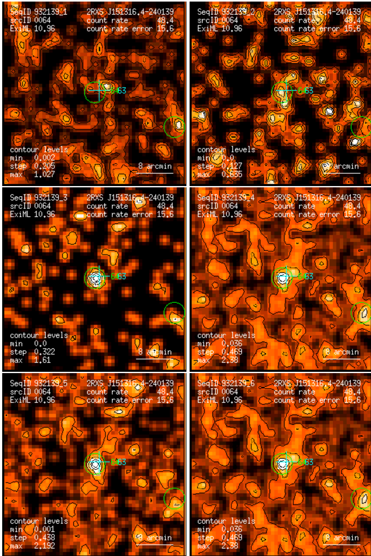
Figure 64: RASS 932139: detection 0064: band rate images, Gaussian filter: (1) PSPC channels 11 – 41, (2) 52 – 90, (3) 91 – 201, (4) 11 – 235, (5) 52 – 201, (6) 11 – 201. Broad band rates in counts/ks. Band rate contour levels in counts/ks/arcmin 2 .
