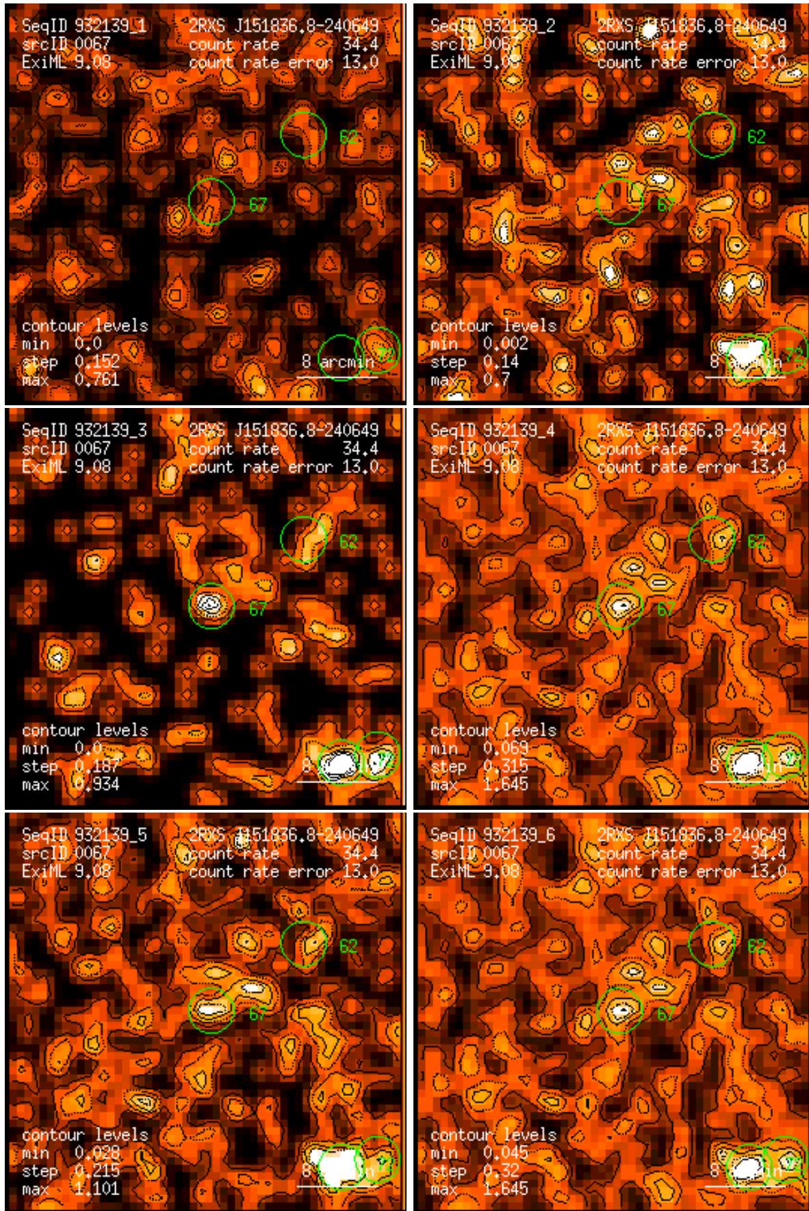
Figure 67: RASS 932139: detection 0067: band rate images, Gaussian filter: (1) PSPC channels 11 – 41, (2) 52 – 90, (3) 91 – 201, (4) 11 – 235, (5) 52 – 201, (6) 11 – 201. Broad band rates in counts/ks. Band rate contour levels in counts/ks/arcmin 2 .
