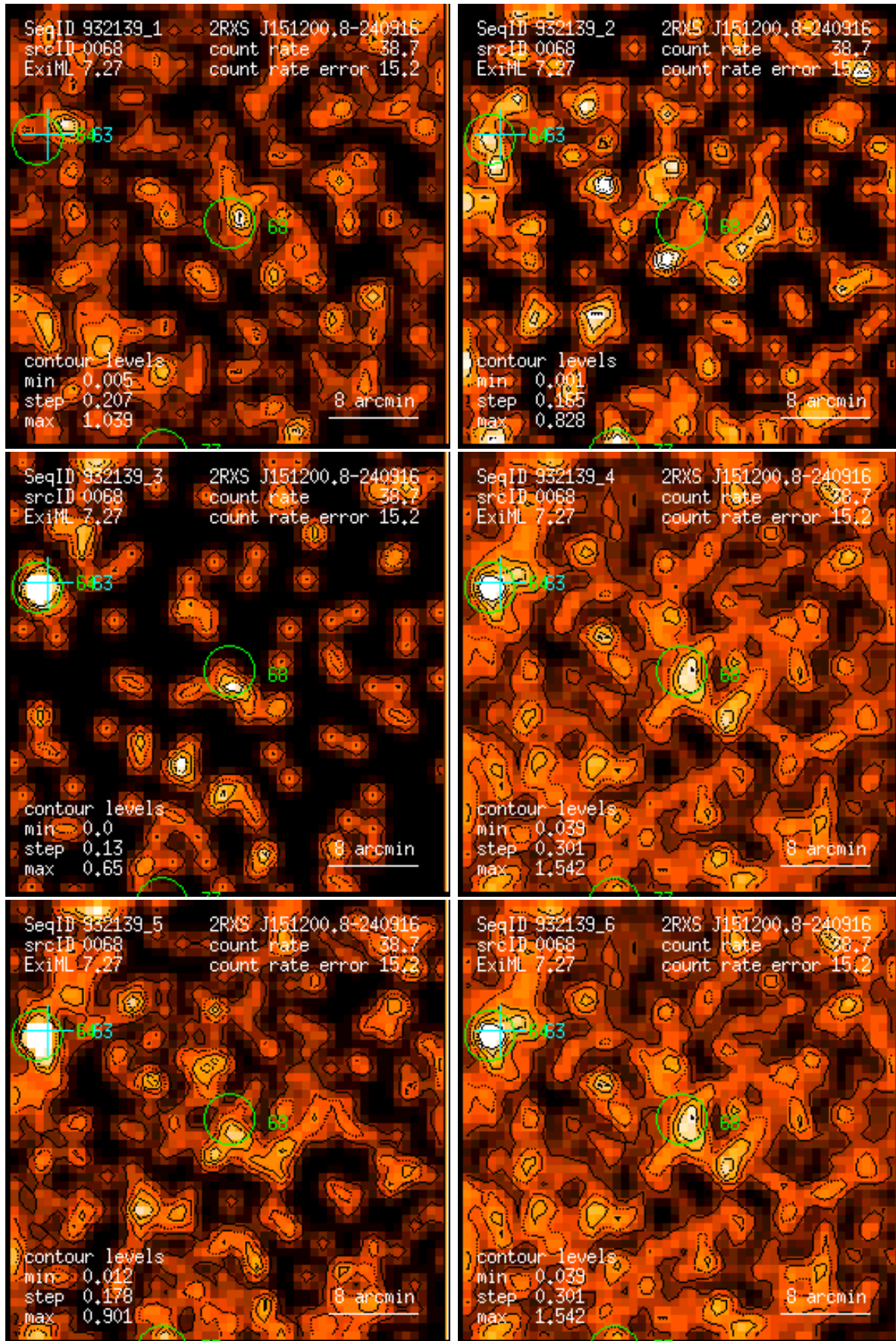
Figure 68: RASS 932139: detection 0068: band rate images, Gaussian filter: (1) PSPC channels 11 – 41, (2) 52 – 90, (3) 91 – 201, (4) 11 – 235, (5) 52 – 201, (6) 11 – 201. Broad band rates in counts/ks. Band rate contour levels in counts/ks/arcmin 2 .
