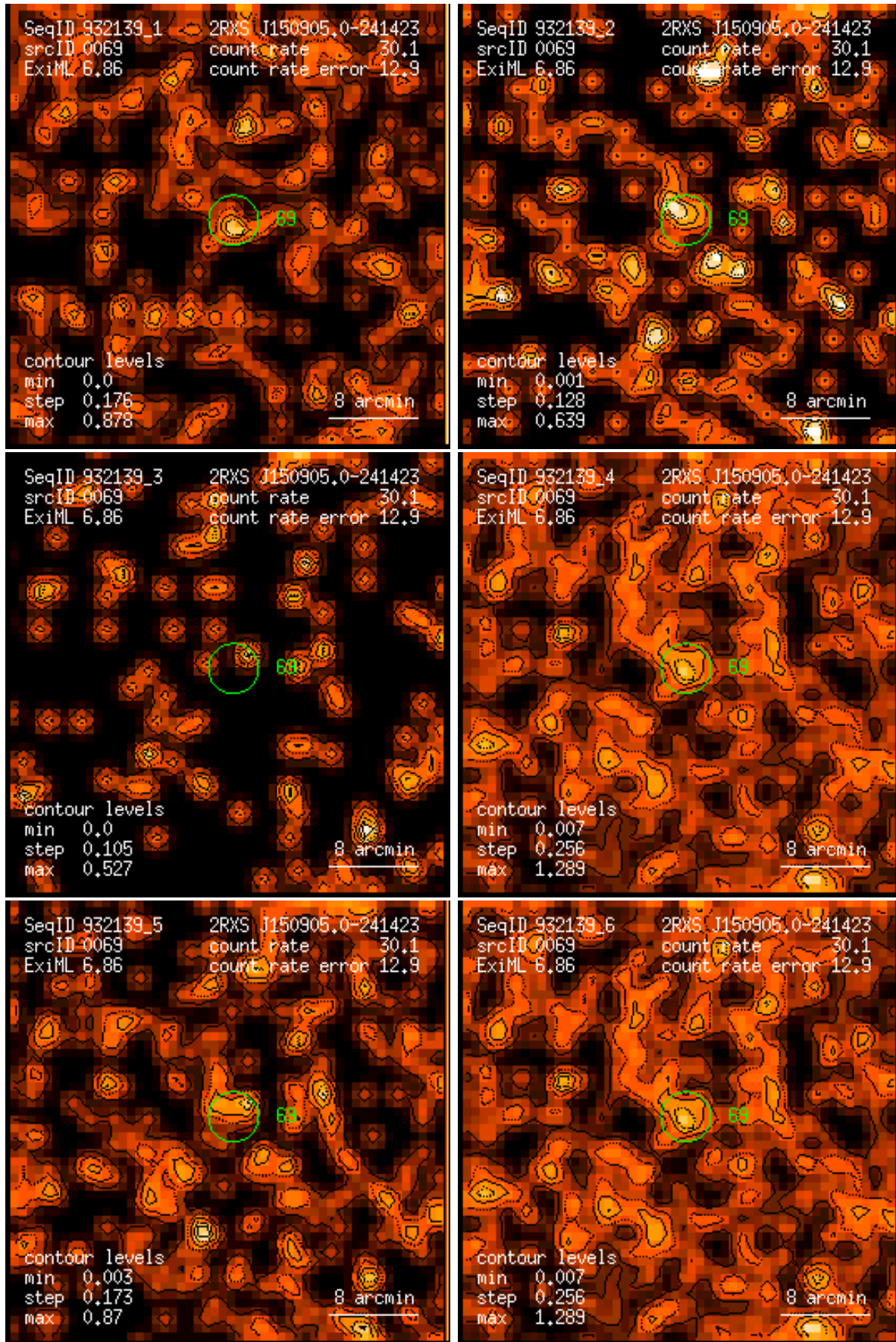
Figure 69: RASS 932139: detection 0069: band rate images, Gaussian filter: (1) PSPC channels 11 – 41, (2) 52 – 90, (3) 91 – 201, (4) 11 – 235, (5) 52 – 201, (6) 11 – 201. Broad band rates in counts/ks. Band rate contour levels in counts/ks/arcmin 2 .
