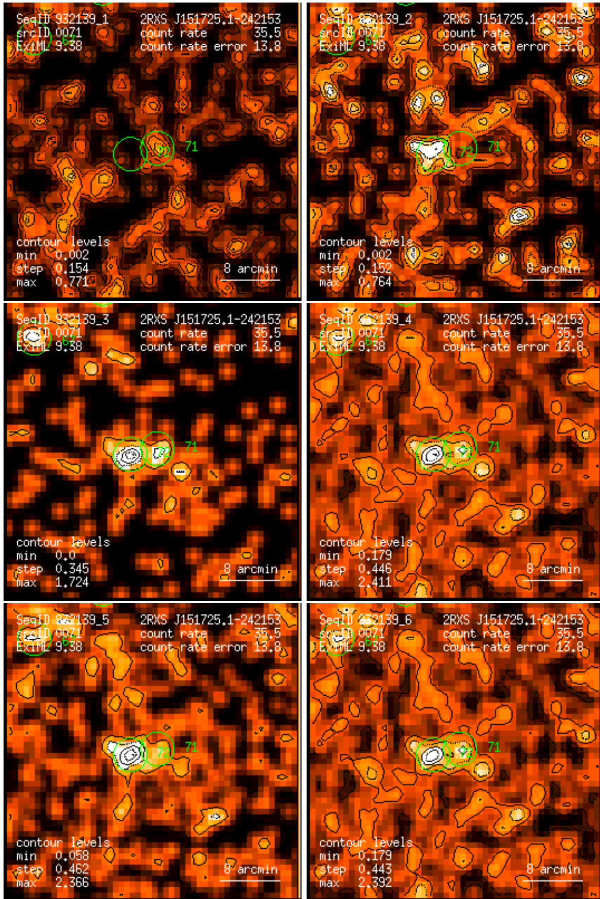
Figure 71: RASS 932139: detection 0071: band rate images, Gaussian filter: (1) PSPC channels 11 – 41, (2) 52 – 90, (3) 91 – 201, (4) 11 – 235, (5) 52 – 201, (6) 11 – 201. Broad band rates in counts/ks. Band rate contour levels in counts/ks/arcmin 2 .
