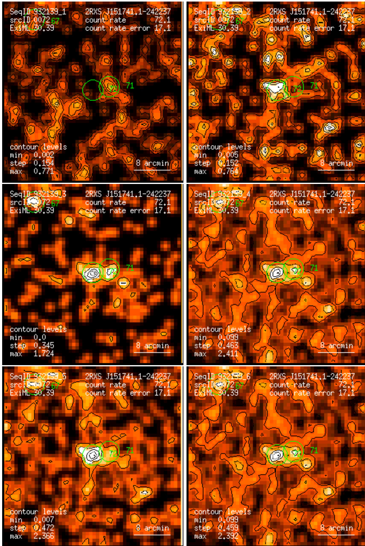
Figure 72: RASS 932139: detection 0072: band rate images, Gaussian filter: (1) PSPC channels 11 – 41, (2) 52 – 90, (3) 91 – 201, (4) 11 – 235, (5) 52 – 201, (6) 11 – 201. Broad band rates in counts/ks. Band rate contour levels in counts/ks/arcmin 2 .
