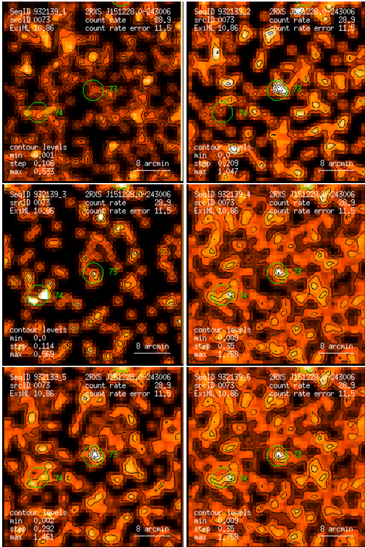
Figure 73: RASS 932139: detection 0073: band rate images, Gaussian filter: (1) PSPC channels 11 – 41, (2) 52 – 90, (3) 91 – 201, (4) 11 – 235, (5) 52 – 201, (6) 11 – 201. Broad band rates in counts/ks. Band rate contour levels in counts/ks/arcmin 2 .
