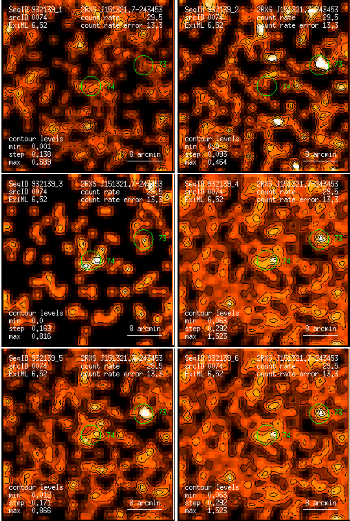
Figure 74: RASS 932139: detection 0074: band rate images, Gaussian filter: (1) PSPC channels 11 – 41, (2) 52 – 90, (3) 91 – 201, (4) 11 – 235, (5) 52 – 201, (6) 11 – 201. Broad band rates in counts/ks. Band rate contour levels in counts/ks/arcmin 2 .
