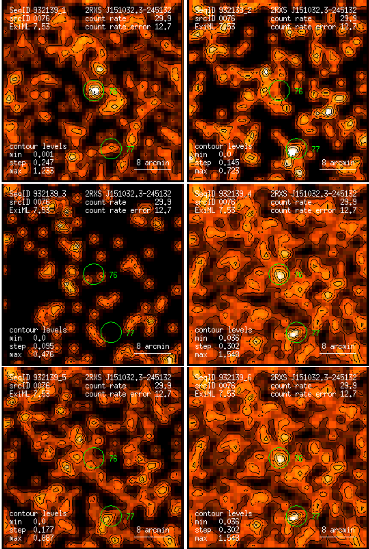
Figure 76: RASS 932139: detection 0076: band rate images, Gaussian filter: (1) PSPC channels 11 – 41, (2) 52 – 90, (3) 91 – 201, (4) 11 – 235, (5) 52 – 201, (6) 11 – 201. Broad band rates in counts/ks. Band rate contour levels in counts/ks/arcmin 2 .
