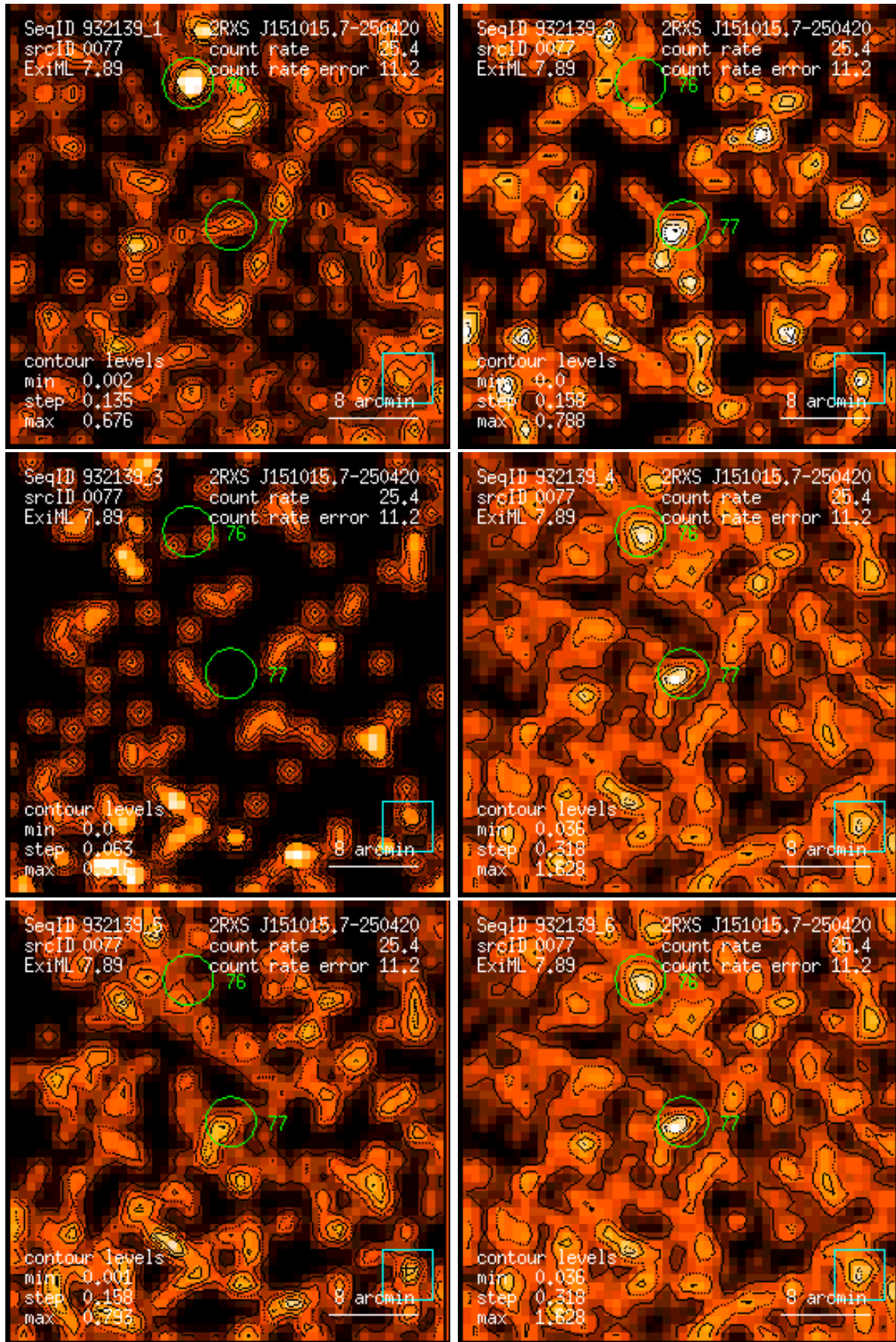
Figure 77: RASS 932139: detection 0077: band rate images, Gaussian filter: (1) PSPC channels 11 – 41, (2) 52 – 90, (3) 91 – 201, (4) 11 – 235, (5) 52 – 201, (6) 11 – 201. Broad band rates in counts/ks. Band rate contour levels in counts/ks/arcmin 2 .
