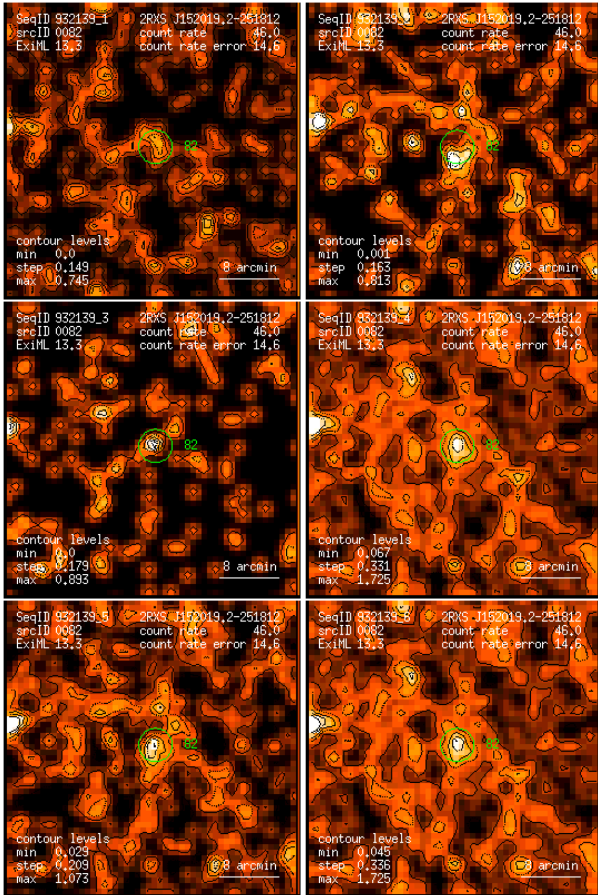
Figure 82: RASS 932139: detection 0082: band rate images, Gaussian filter: (1) PSPC channels 11 – 41, (2) 52 – 90, (3) 91 – 201, (4) 11 – 235, (5) 52 – 201, (6) 11 – 201. Broad band rates in counts/ks. Band rate contour levels in counts/ks/arcmin 2 .
