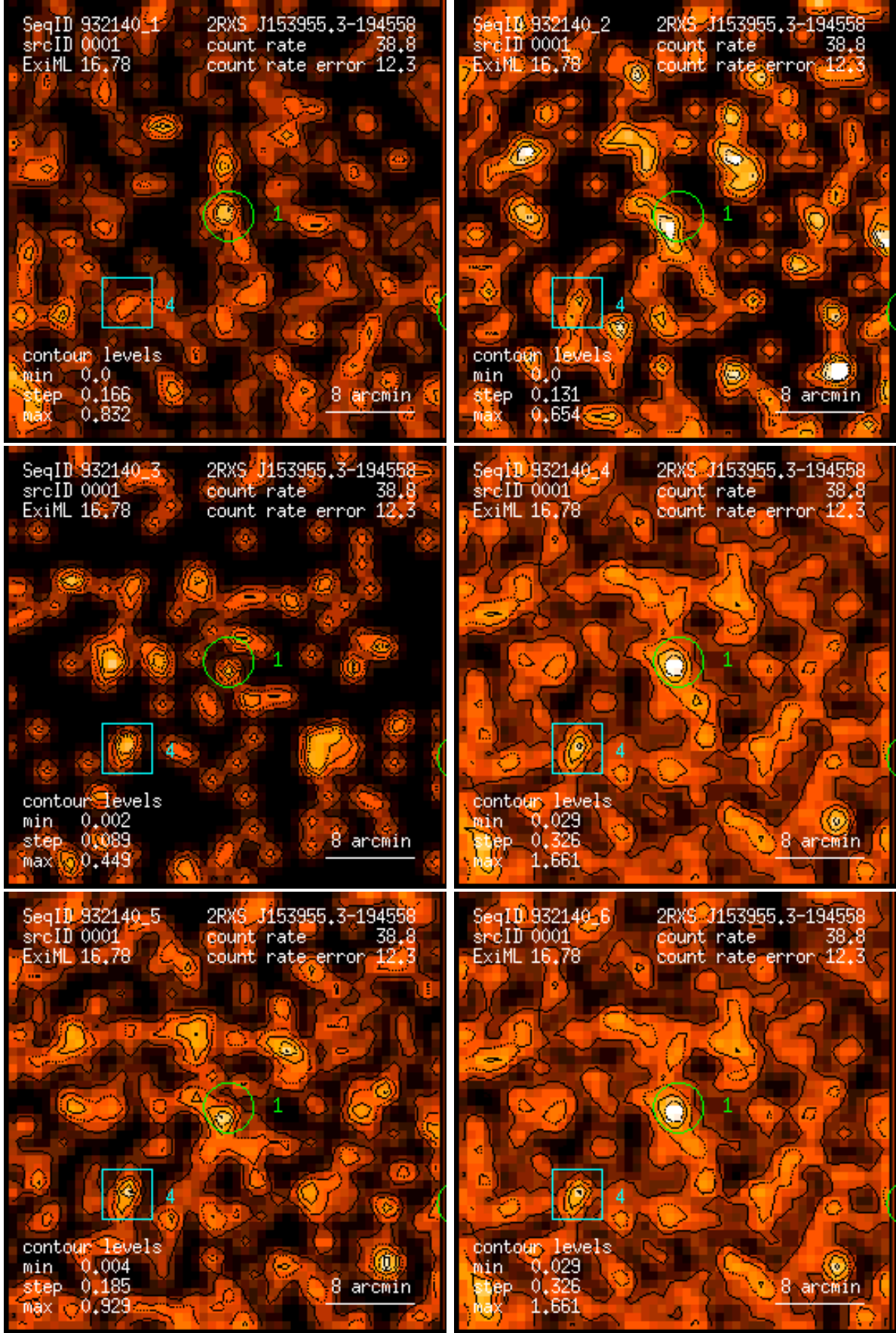
Figure 1: RASS 932140: detection 0001: band rate images, Gaussian filter: (1) PSPC channels 11 – 41, (2) 52 – 90, (3) 91 – 201, (4) 11 – 235, (5) 52 – 201, (6) 11 – 201. Broad band rates in counts/ks. Band rate contour levels in counts/ks/arcmin 2 .
