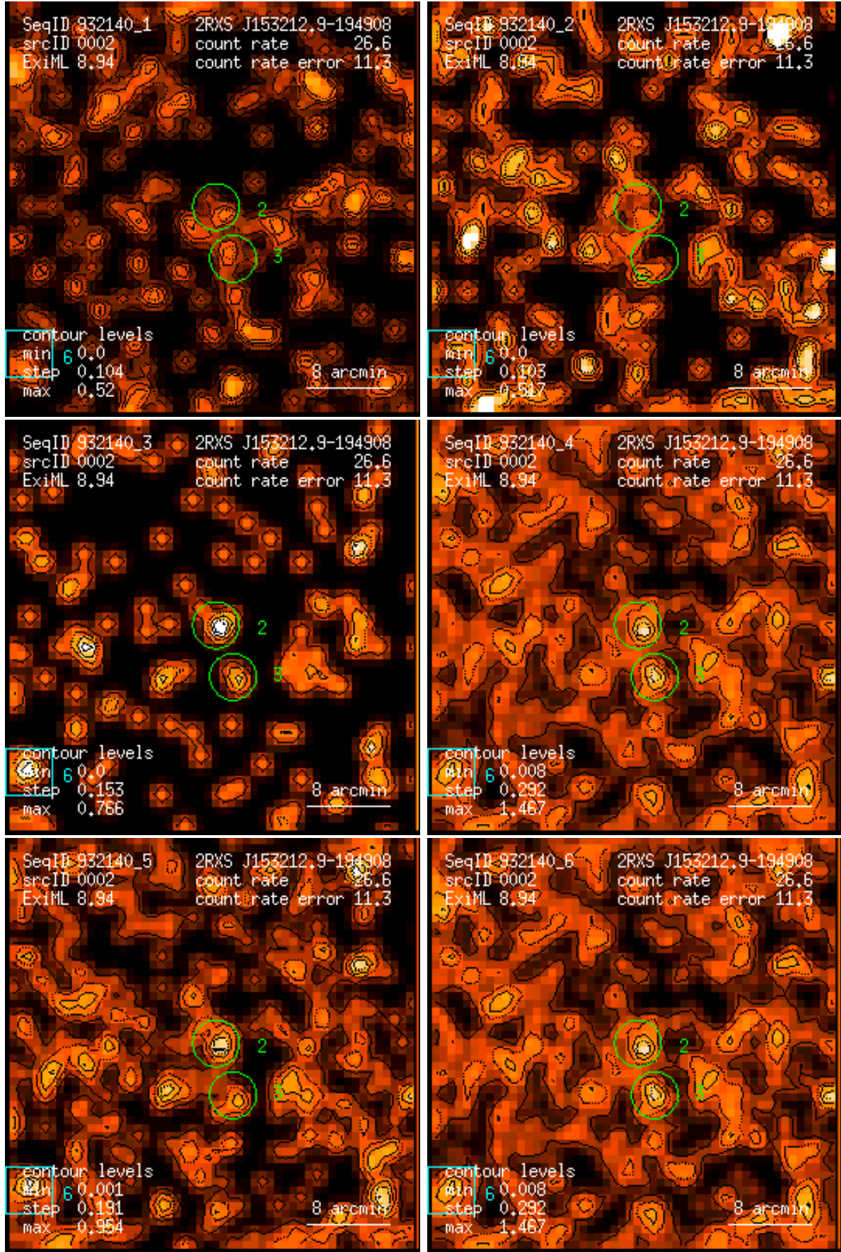
Figure 2: RASS 932140: detection 0002: band rate images, Gaussian filter: (1) PSPC channels 11 – 41, (2) 52 – 90, (3) 91 – 201, (4) 11 – 235, (5) 52 – 201, (6) 11 – 201. Broad band rates in counts/ks. Band rate contour levels in counts/ks/arcmin 2 .
