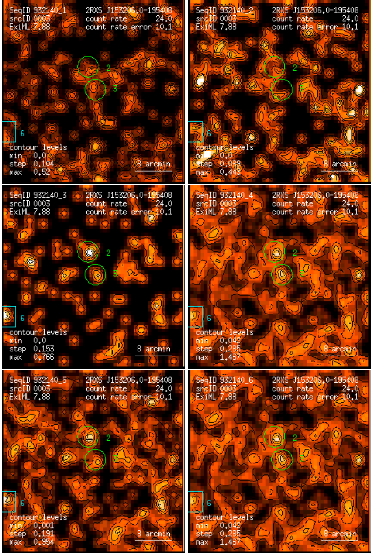
Figure 3: RASS 932140: detection 0003: band rate images, Gaussian filter: (1) PSPC channels 11 – 41, (2) 52 – 90, (3) 91 – 201, (4) 11 – 235, (5) 52 – 201, (6) 11 – 201. Broad band rates in counts/ks. Band rate contour levels in counts/ks/arcmin 2 .
