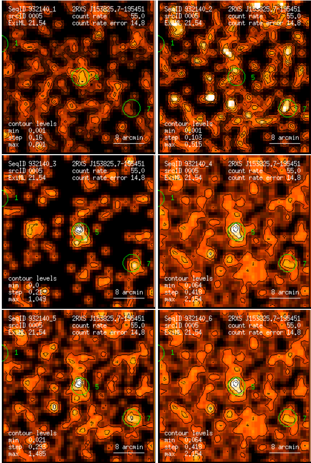
Figure 5: RASS 932140: detection 0005: band rate images, Gaussian filter: (1) PSPC channels 11 – 41, (2) 52 – 90, (3) 91 – 201, (4) 11 – 235, (5) 52 – 201, (6) 11 – 201. Broad band rates in counts/ks. Band rate contour levels in counts/ks/arcmin 2 .
