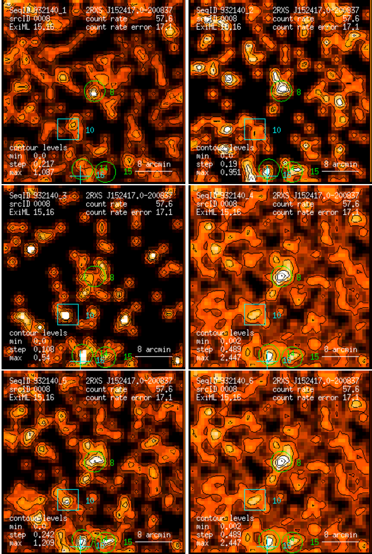
Figure 8: RASS 932140: detection 0008: band rate images, Gaussian filter: (1) PSPC channels 11 – 41, (2) 52 – 90, (3) 91 – 201, (4) 11 – 235, (5) 52 – 201, (6) 11 – 201. Broad band rates in counts/ks. Band rate contour levels in counts/ks/arcmin 2 .
