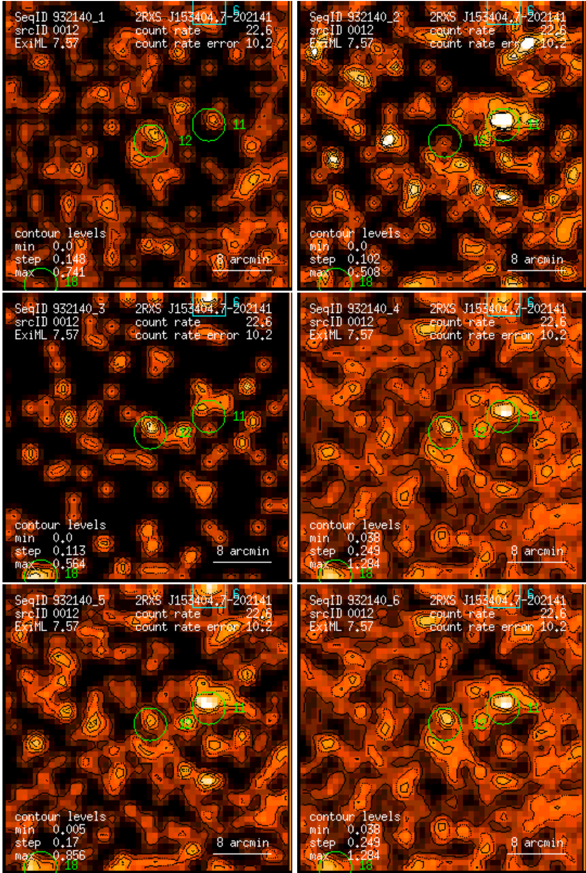
Figure 12: RASS 932140: detection 0012: band rate images, Gaussian filter: (1) PSPC channels 11 – 41, (2) 52 – 90, (3) 91 – 201, (4) 11 – 235, (5) 52 – 201, (6) 11 – 201. Broad band rates in counts/ks. Band rate contour levels in counts/ks/arcmin 2 .
