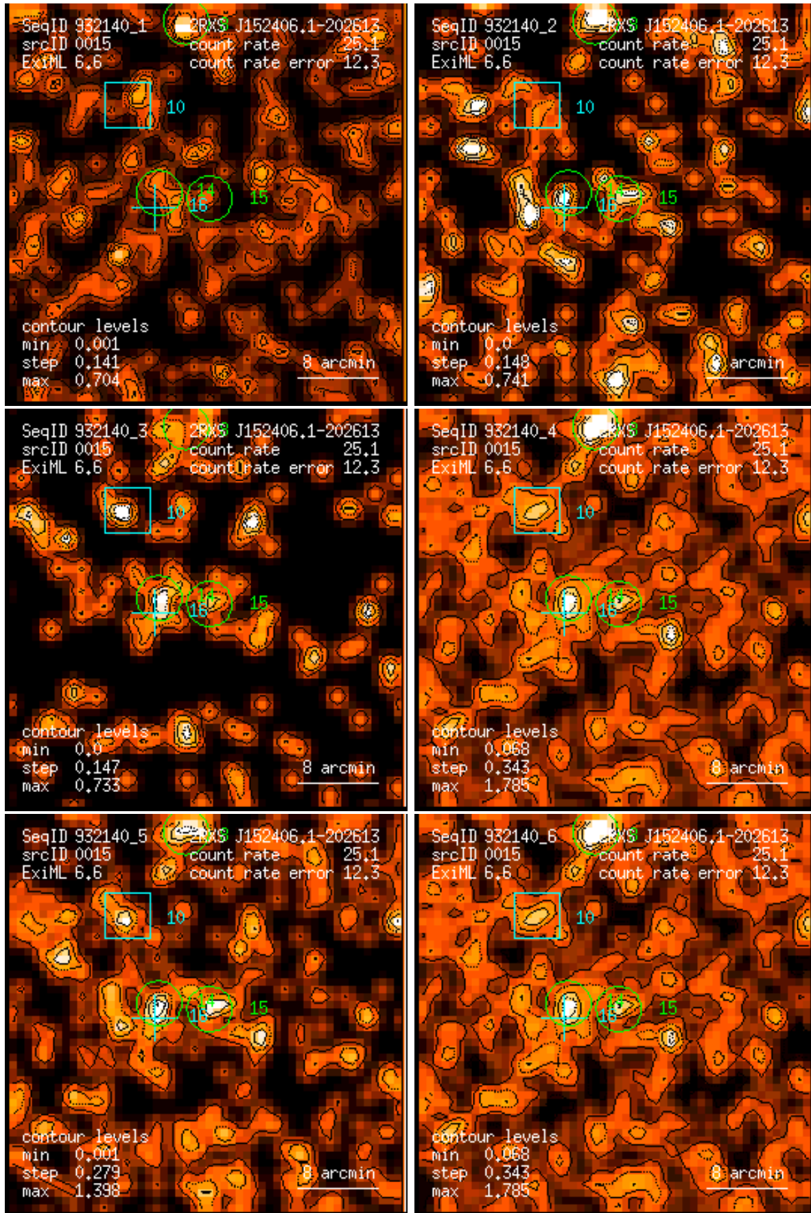
Figure 15: RASS 932140: detection 0015: band rate images, Gaussian filter: (1) PSPC channels 11 – 41, (2) 52 – 90, (3) 91 – 201, (4) 11 – 235, (5) 52 – 201, (6) 11 – 201. Broad band rates in counts/ks. Band rate contour levels in counts/ks/arcmin 2 .
